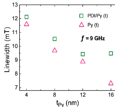
Fig. 5 Linewidth values of PDI/Py and reference Py films for all the thicknesses of Py at f = 9 GHz.
