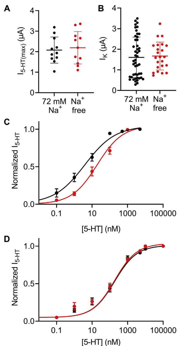
Figure 3. Allosteric effect of sodium ions on the 5-HT 1A receptor. A , the maximal amplitude of I_{5\text{-HT}} , evoked by 5 \mu\text{M} 5-HT in 72 mM \text{Na}^+ solution (black) and in \text{Na}^+ -free solution (red). Each data point represents one oocyte, and the mean ( \pm\text{SD} ) is shown as a horizontal line. The data at the two conditions are not significantly different (unpaired t test, p = 0.79 ). B , basal I_K from experiments in 72 mM \text{Na}^+ solution (black) described for Figure 1 and in \text{Na}^+ -free solution (red). Each data point represents one oocyte, and the mean ( \pm\text{SD} ) is shown as horizontal lines. The data at the two conditions are not significantly different (unpaired t test, p = 0.76 ). C and D , DR curves assembled from various experiments conducted on wt 5-HT 1A receptor ( C ) or Asp92Asn mutant ( D ) at 72 mM \text{Na}^+ solution (black circles) and in \text{Na}^+ -free solution (red circles). Each point represents the mean ( \pm\text{SEM} ) from 8 to 31 oocytes. The solid black and red lines were generated as described previously for Figure 1. The \text{EC}_{50} values obtained for the two graphs at C are significantly different ( p = 0.016 ). The \text{EC}_{50} values obtained for the two graphs at D are not significantly different ( p = 0.15 ). 5-HT, 5-hydroxytryptamine; DR, dose response; I_{5\text{-HT}} , 5-HT-induced \text{K}^+ current.
