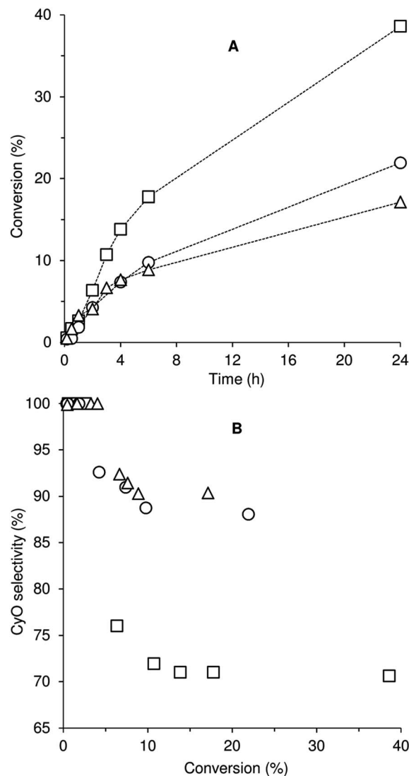
Fig. 2 cis -Cyclooctene epoxidation with TBHP D at 55 °C (DCE as cosolvent) using compounds 1 (□), 2 (○) and 3 (△): (A) conversion of Cy as a function of time and (B) selectivity of CyO as a function of Cy conversion. The dashed lines are visual guides.
