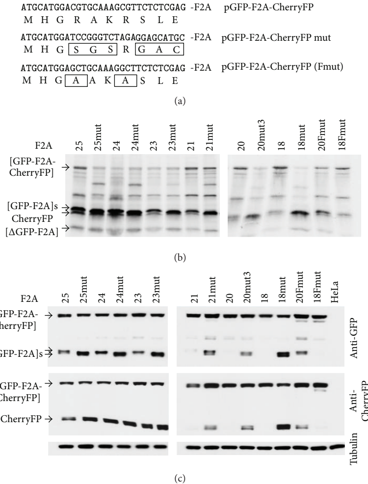
FIGURE 3: Effect of -RAKRSLE- to -SGSRGAC- substitution immediately upstream of F2A on cleavage efficiency of pGFP-F2A-Cherry constructs with F2As of 25–18aa. Parental pGFP-F2A-Cherry constructs and their mutant versions (mut or Fmut) (mutated residues are boxed, (a)) were used to coexpress GFP and CherryFP proteins from a single ORF in vitro using coupled transcription/translation rabbit reticulocyte lysate system (b) and transfected HeLa cells (c). For TnT , reticulocyte lysates were programmed with 20 ng of plasmid DNA, and translation products were resolved by the 12% SDS-PAGE. For in vivo studies, HeLa cells were transfected with 1.5 \mu g of plasmid DNA and harvested 30 h after transfection. Cells were lysed in RIPA buffer, and equal amounts of total protein for each transfection were loaded onto 12% SDS-PAGE gel. The proteins were transferred onto a nitrocellulose membrane, blocked in PBS containing 5% milk, and probed with anti-GFP (upper blot) and anti-CherryFP (middle blot) antibodies overnight at 4°C. Detection of bound primary antibody was achieved by using respective secondary antibodies, followed by ECL detection. All experiments were done in triplicate.
