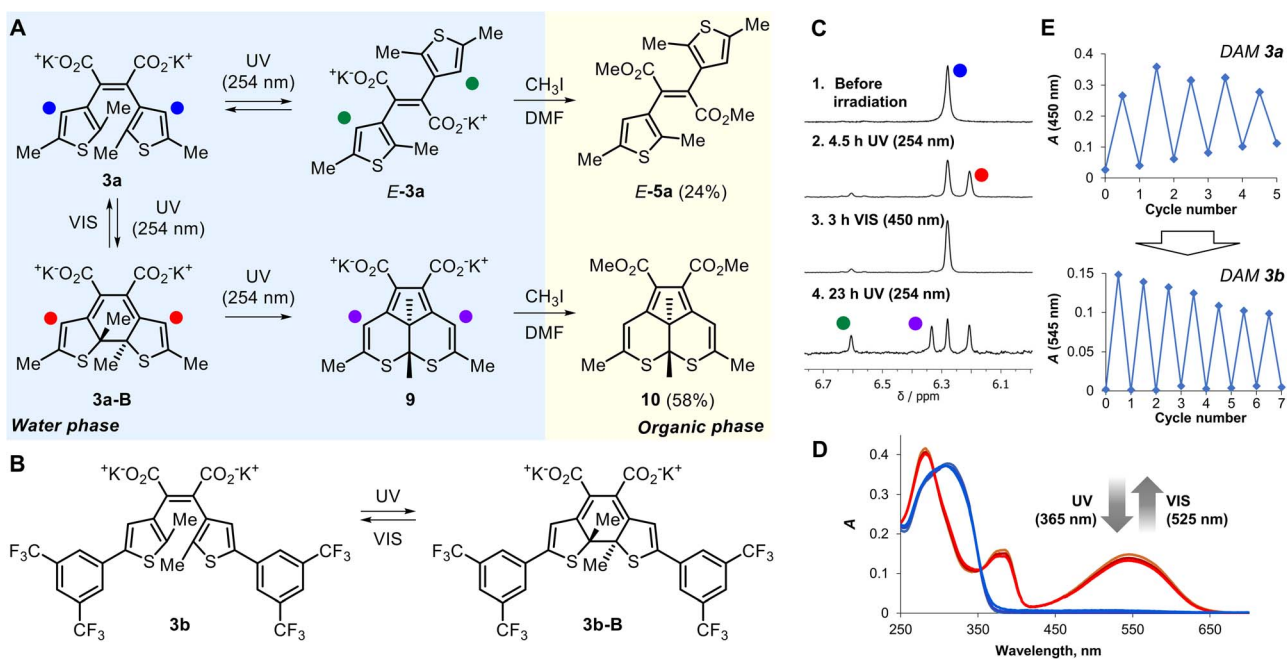
Fig. 2 Photoreactions of DAMs 3a (A) and 3b (B). 1 H NMR spectra of 3a under irradiation with UV and visible light in D 2 O (C). Changes in UV-Vis spectra of 3b during three cycles of cyclization–cycloreversion in 1 : 1 MeCN/H 2 O (D). Multiple photoswitching of DAMs 3a and 3b in H 2 O and MeCN/H 2 O (buffer pH = 7.00), respectively (E).
