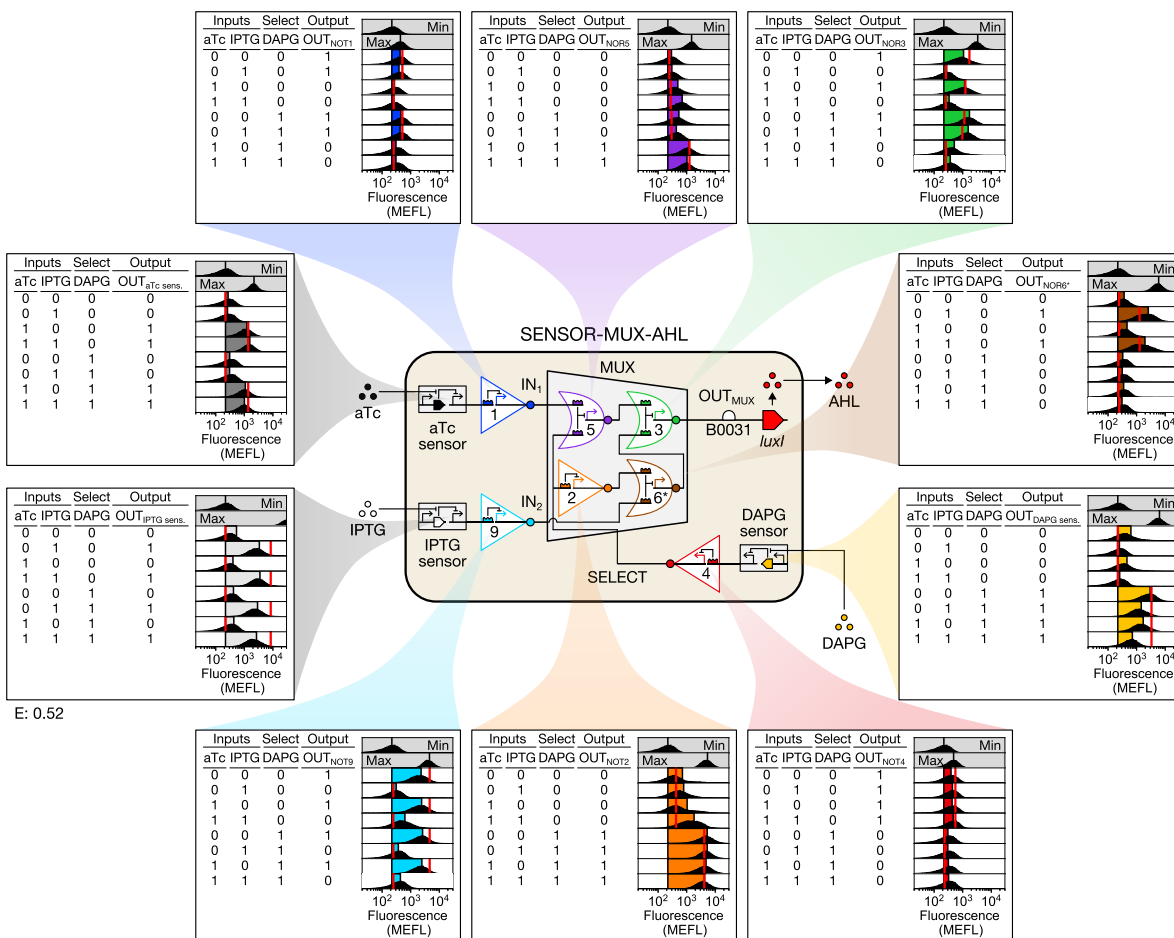
Figure 4. Linking the MUX to chemical sensors and a cell-cell communication system.
