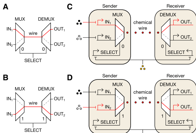
Figure 1. Electronic and biological channel selectors.
