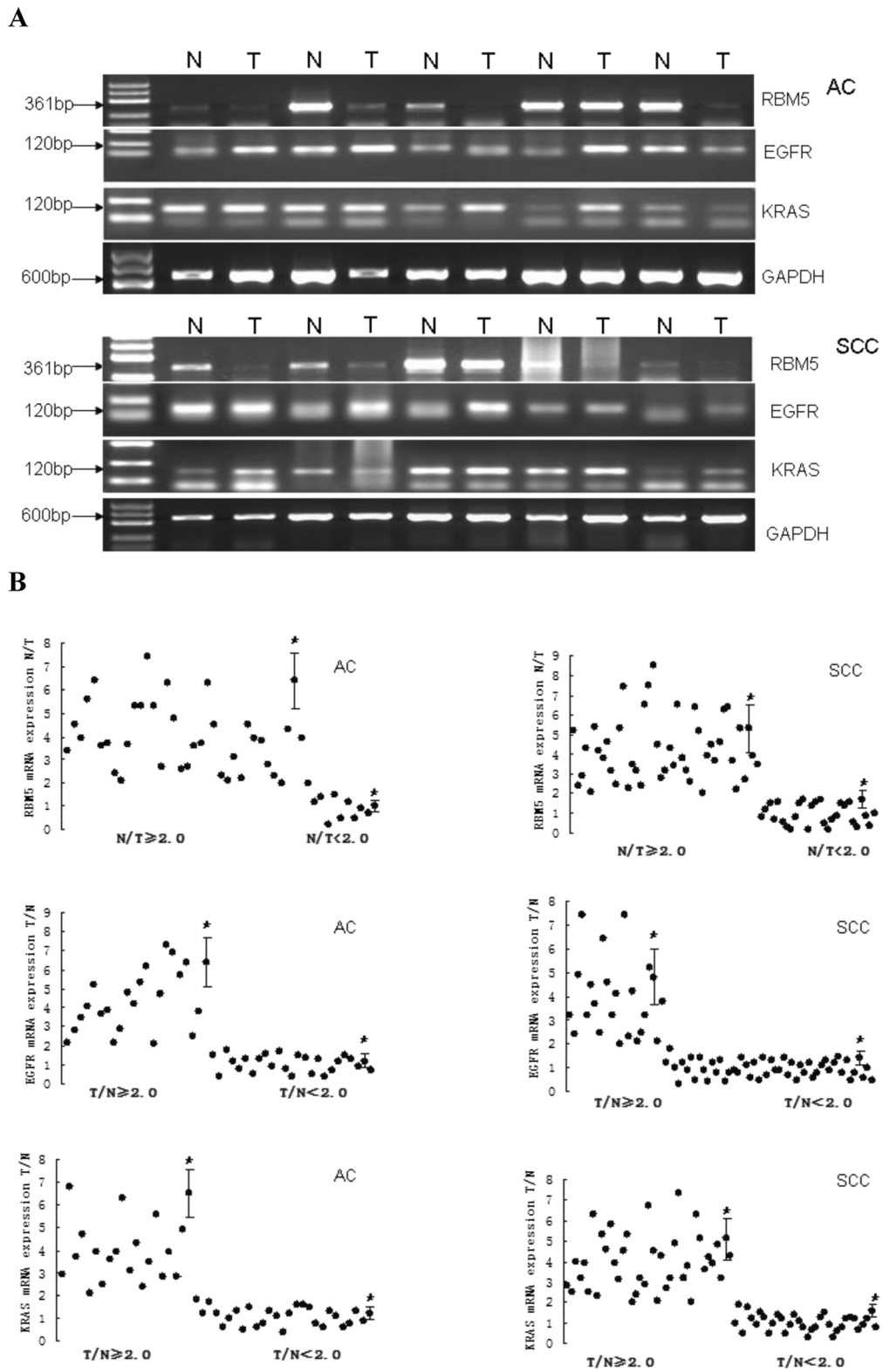
Figure 1 Expression of RBM5, EGFR and KRAS mRNA in NSCLC. A, Agarose gel of semi-quantitative RT-PCR data of RBM5, EGFR, and KRAS mRNA expression in representative NSCLC and non-tumor specimens. Total RNA was isolated and subjected to semi-quantitative RT-PCR and quantified using Quantity One software. B, Quantitative data from A. * p < 0.05 compared to the normal tissues using Wilcoxon signed rank test.
