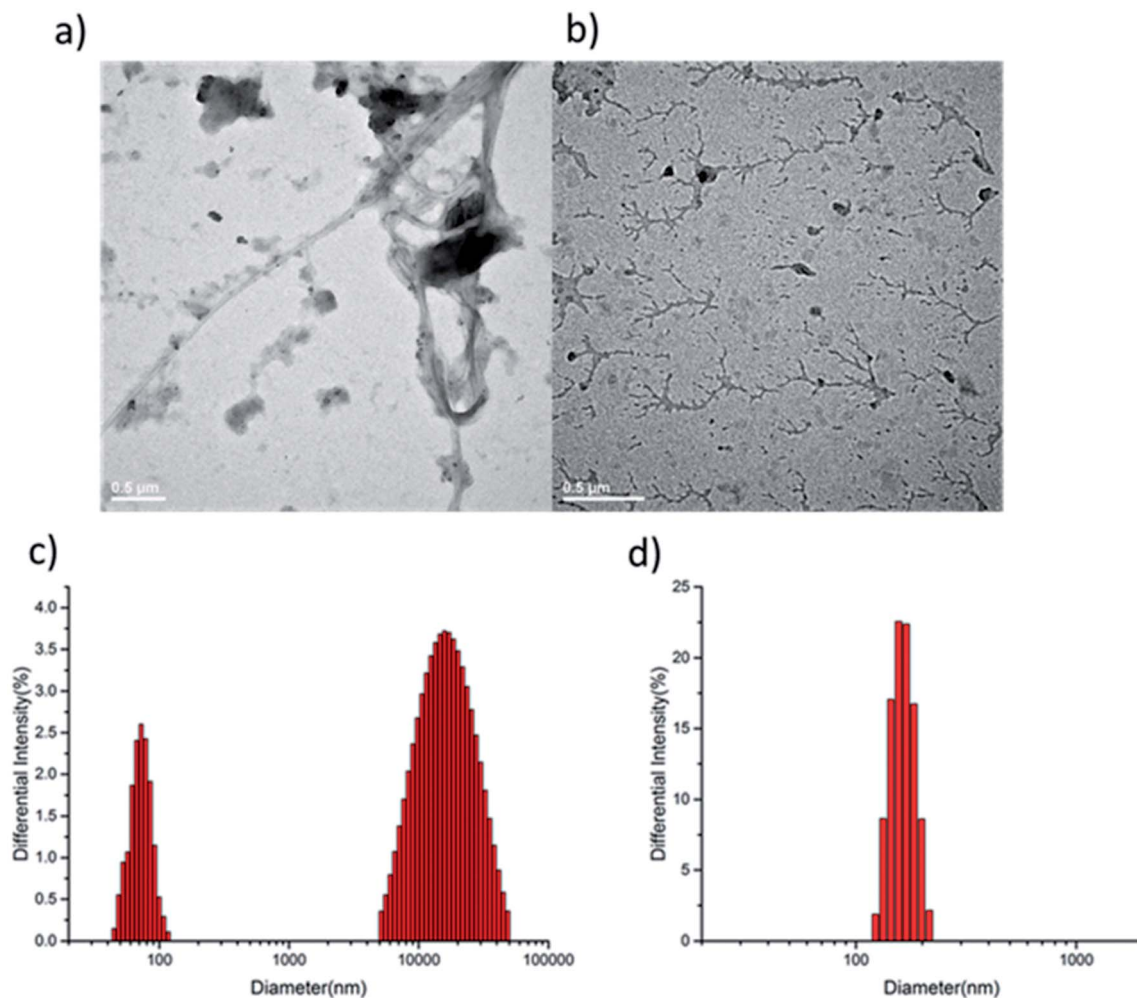
Fig. 3 TEM images of the supramolecular polymer (a) HCDV-2CB[8] negative stained by Phosphotungstic acid and (b) PCDV-2CB[8] (40 \mu M) in water; DLS results of (c) HCDV-2CB[8] and (d) PCDV-2CB[8] (0.5 mM) in water.
