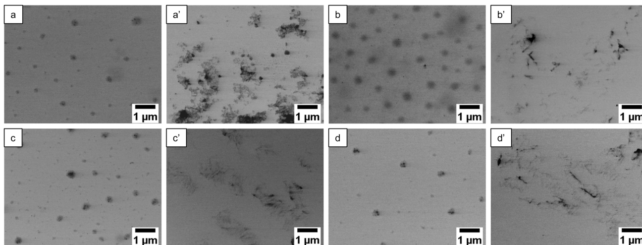
Fig. 4 STEM images of Se 1 G before sonication of (a) 0.5, (b) 1.5, (c) 3.0, and (d) 5.0 mol% diselenide content. The images after 10 min sonication (a'), (b'), (c'), and (d') correspond to (a), (b), (c), and (d), respectively. Sonication was carried out in an ice bath at 30% amplitude for 10 min.
