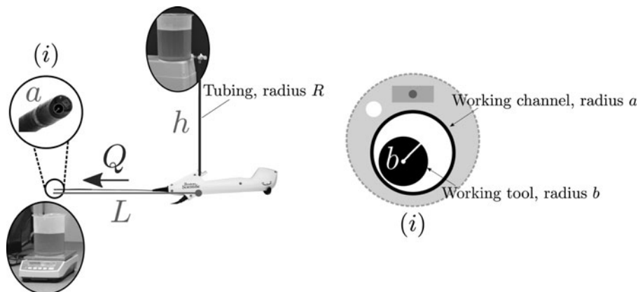
FIG. 1. A schematic of the experimental setup labeled with variables and parameters used in the theoretical model. The top of the fluid is at height h above the scope and flows through tubing of radius R . The ureteroscope working channel is of radius a and length L . The flow rate, Q , is measured using a mass balance. Inset figure (i) demonstrates a cross-sectional view of the scope, with the working channel containing a working tool of radius b .
