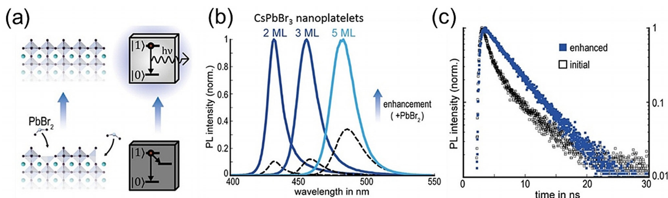
Figure 6. a) Schematic illustration showing the post-synthetic surface repair of CsPbBr 3 NPIs by chemical treatment with a PbBr 2 solution to improve their photoluminescence efficiency. b) Photoluminescence spectra of pristine (black dashed lines) and surface-repaired (normalized, solid lines) colloidal dispersions of CsPbBr 3 NPIs with three different thicknesses. The enhancement clearly increases as the thickness of the NPIs decreases, which suggests that the defects are more effective as the surface to volume ratio increases. c) Time-resolved photoluminescence spectra of a 3-monolayer NPI dispersion before (open black squares) and after surface repair (filled blue squares). (a,b,c) are reproduced from Ref. [14c] with permission the under Creative Common CC-BY license. Copyright 2018, American Chemical Society.
