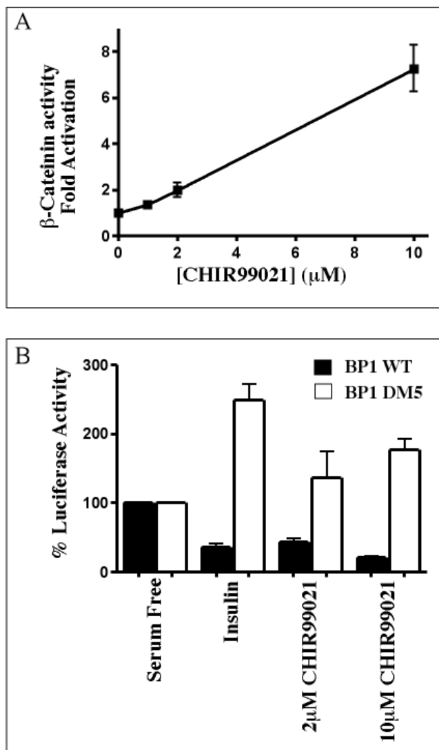
Figure 7 CHIR99021 regulates both \beta -catenin activity and TIRE containing promoter activity. H4IIE cells were transfected with TOPFlash (A) or alternatively with BP-1 WT or BP-1 DM5 (B) reporter constructs. Cells were incubated for 24 h with 10 nM insulin or CHIR99021 at the concentrations shown, prior to lysis and luciferase assays as described in materials and methods. Results are presented as fold induction relative to basal luciferase activity (no inhibitor) (A) or % luciferase activity relative to basal (serum free) luciferase expression (B) and are the means \pm standard error of at least two experiments performed in triplicate. The basal activity of BP-1 WT and BP-1 DM5 is not significantly different.
