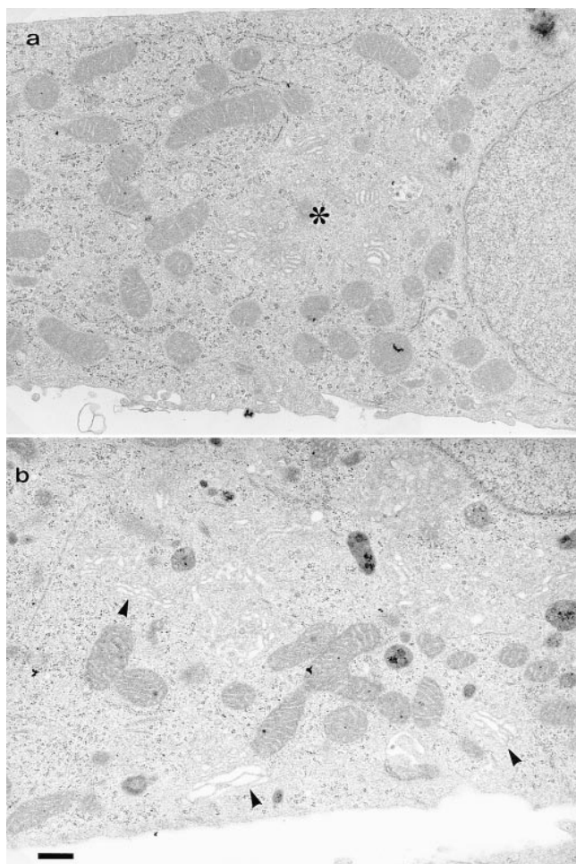
Figure 7. In 201-F-treated cells, the Golgi fragments are composed of stacked cisternae. The Golgi fragments were visualized by electron microscopy in control cells ( a ) or after cells were treated for 60 min with 201-F ( b ). Cells were fixed with 3% glutaraldehyde in sodium phosphate buffer, post-fixed in 1% osmic acid, embedded in Epon, and ultrathin sections were counterstained with uranyl acetate and lead citrate. In a typical control cell, the Golgi complex was observed as a condensed organelle ( asterix ) located close to the nucleus. 201-F-treated cells exhibited Golgi fragments with stacked cisternae ( arrowheads ). Bar, 0.5 \mu\text{m} .
