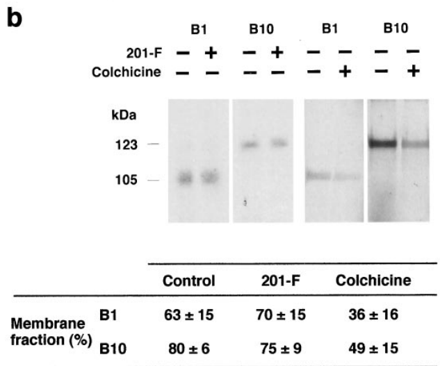
Figure 9. Stable MTs are involved in the transport of membrane proteins to the basolateral surface of WIF-B cells. In a , cells were treated for times ranging between 1 and 10 h with 10 \mu M colchicine. To minimize background fluorescence, soluble tubulin was extracted by permeabilizing cells with 0.15% Triton X-100 in MT-stabilizing buffer (1 min, 37°C). Cells were then fixed, processed for immunofluorescence labeling of \alpha -tubulin, and examined in a fluorescence microscope. Short MTs were still observed in cells treated for up to 4 h with colchicine (arrowheads), but could not be detected after 10 h of treatment. When present, bile canaliculi ( b.c. ) are identified. Bar, 10 \mu M. b shows the effects of 1-h treatment with 201-F and 10-h treatment with colchicine on basolateral membrane expression of B1 and B10 proteins. Newly synthesized proteins were radiolabeled and chased for 1 h in the presence of 201-F or colchicine, and were then subjected to surface biotinylation. Total B1 and B10 were first immunoprecipitated from cell lysates, and then the biotinylated fractions were precipitated using streptavidin-agarose. Samples were analyzed by SDS-PAGE, fluorography and densitometry. Membrane fractions of B1 and B10 are the mean \pm SD of three determinations.
