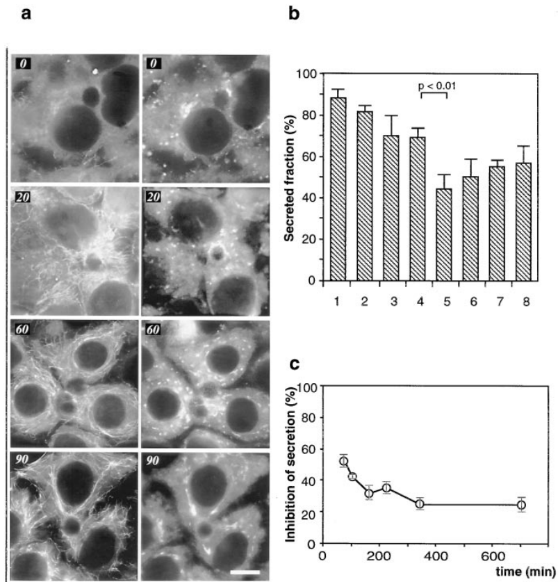
Figure 8. Neither Golgi fragmentation nor a direct effect of 201-F on Golgi membranes are responsible for the inhibitory effect of 201-F on protein secretion. In a , cells were treated for 1.5 h with 10 \mu M nocodazole. Nocodazole was then washed out to allow reconstitution of the MT network and compaction of Golgi fragments. At various times ranging from 0 to 90 min after drug removal, cells were fixed, processed for double immunofluorescence labeling of \alpha -tubulin ( left side ) and albumin ( right side ), and examined in a fluorescence microscope. Bar, 10 \mu m. b shows the mean secreted fractions \pm SEM of albumin after 1-h pulse-chase experiments performed in the following conditions: (1) no treatment; (2) 10 \mu M nocodazole pretreatment (1 h) and depletion of methionine and cysteine in the presence of nocodazole (30 min), radiolabeling (15 min), and chase (60 min) without nocodazole; (3) 10 \mu M nocodazole pretreatment (4 h), depletion (30 min), pulse labeling (15 min), and chase periods (60 min) in the presence of nocodazole; (4) 10 \mu M nocodazole pretreatment (4 h), adding 25 \mu M 201-F during depletion (30 min), pulse labeling (15 min), and chase period (60 min); (5–7) Depletion (30 min), pulse labeling (15 min), and chase (60 min) in the presence of 25 \mu M 201-F (5), 10 \mu M nocodazole (6), or 10 \mu M taxol (7); (8) 10 \mu M taxol pretreatment (1 h), adding 25 \mu M 201-F during the depletion (30 min), pulse labeling (15 min), and chase period (60 min). Data are the mean \pm SEM of eight (1, 5, 6), four (2), or three experiments (3, 4, 7, 8). Statistical
