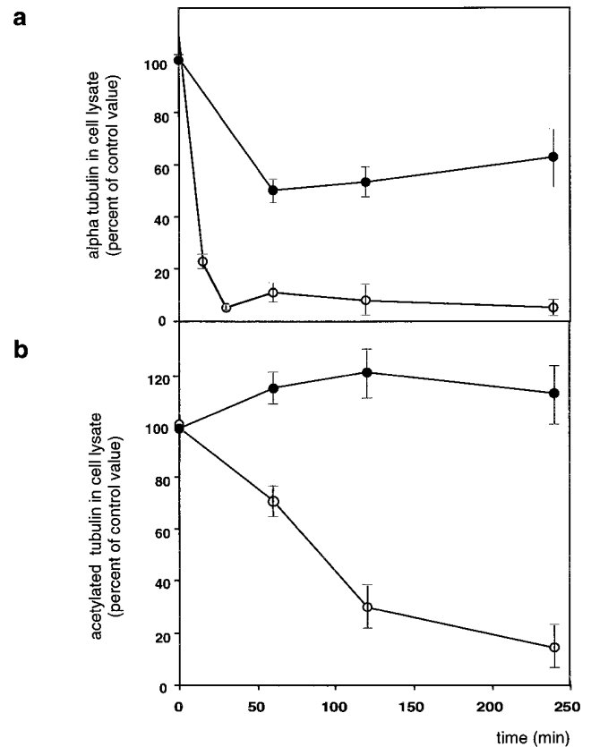
Figure 2. Quantification of \alpha - and acetylated tubulin in MTs during 201-F and nocodazole treatments. WIF-B cells cultured in 12-well plates were incubated for times ranging between 15 min and 4 h with either 25 \mu\text{M} 201-F ( closed symbols ), or 10 \mu\text{M} nocodazole ( open symbols ). At the end of the treatment, soluble tubulin was extracted in MT-stabilizing buffer containing 0.15% Triton X-100 (1 min at 37^\circ\text{C} ) followed by one rinse in Triton-free buffer. Cells were lysed directly using SDS-PAGE sample buffer. Sample lysates and the corresponding cell extracts were analyzed by Western blotting. \alpha - and acetylated tubulin were quantified using enhanced chemiluminescence assay on BioMax films (Eastman Kodak Co.). Data are expressed relative to the MT contents measured in untreated cells. Each value is the mean \pm SD of three to five independent experiments.
