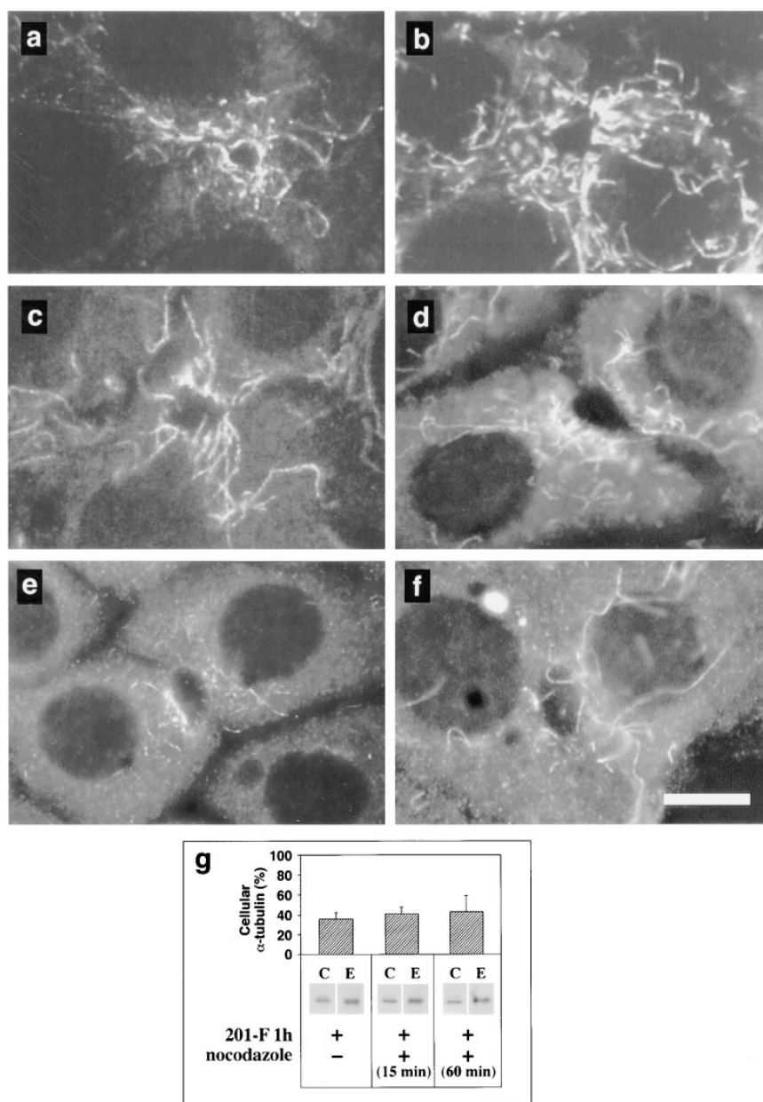
Figure 3. MTs that resist 201-F treatment are stable. In a first series of experiments, control ( a ) and 201-F-treated cells ( b ) were permeabilized using 0.2 mg/ml saponin in Hesper buffer to trigger dilution-induced depolymerization of MTs. MTs were labeled with antibodies to acetylated tubulin, and were observed by means of confocal microscopy. Images are the superimposition of four equidistant optical sections ( \Delta z = 1.5 \mu\text{m} ). Bar, 10 \mu\text{m} . In a second set of experiments ( c-g ), cells were treated with 25 \mu\text{M} 201-F for 1 h. 10 \mu\text{M} nocodazole was then added into the culture medium for 15 ( d ) or 60 min ( f ). 1-h 201-F and 1h-nocodazole controls are shown in c and e , respectively. Cells were then fixed and processed for the immunofluorescent labeling of \alpha -tubulin ( c-f ). Soluble \alpha -tubulin was also extracted with MT-stabilizing buffer containing 0.15% Triton X-100. Cellular (C) and extracted (E) \alpha -tubulin was analyzed by Western blot ( n = 3 ; g ).
