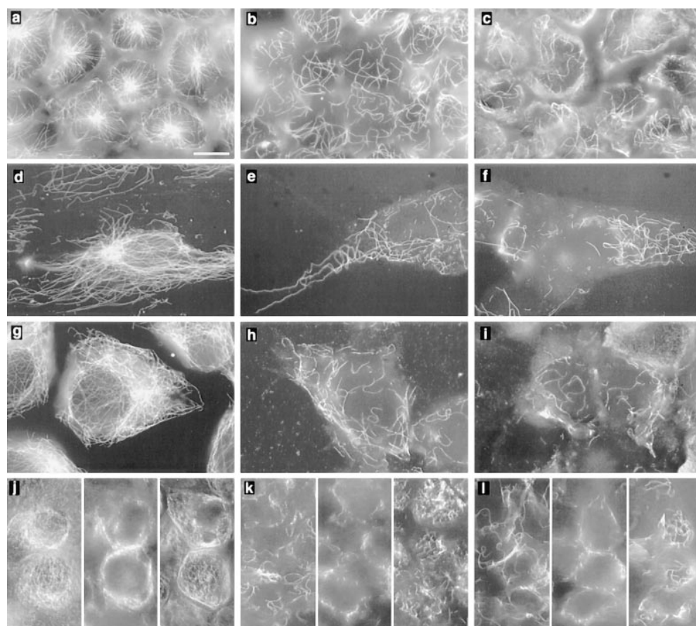
Figure 4. Dynamic MTs are selectively depolymerized by 201-F treatment in fibroblastic and epithelial cells. Fao rat hepatoma cells ( a-c ), human pulmonary fibroblasts ( d-f ), HeLa cells ( g-i ), and MDCK cells ( j-l ) were treated without ( a, d, g, j ) or with 25 \mu M 201-F for 1 h ( b-c, e-f, h-i, k-l ). In some cases, 10 \mu M nocodazole was added into the culture medium for 15 min at the end of the 1-h 201-F treatment ( c, f, i, l ). After three washes with MT-stabilizing buffer, soluble tubulin was extracted with warm MT-stabilizing buffer containing 0.02% Triton X-100 (37°C, 4 \times for 1 min). After fixation (methanol at -20^{\circ} C for 5 min), cells were processed for immunofluorescence labeling of \alpha -tubulin and examined in a fluorescence microscope. For MDCK cells, three optical sections of the same cells were taken near the basal domain ( left ), across the lateral domain ( middle ) and near the apical domain ( right ) in each panel ( j-l ). Bar, 10 \mu m.
