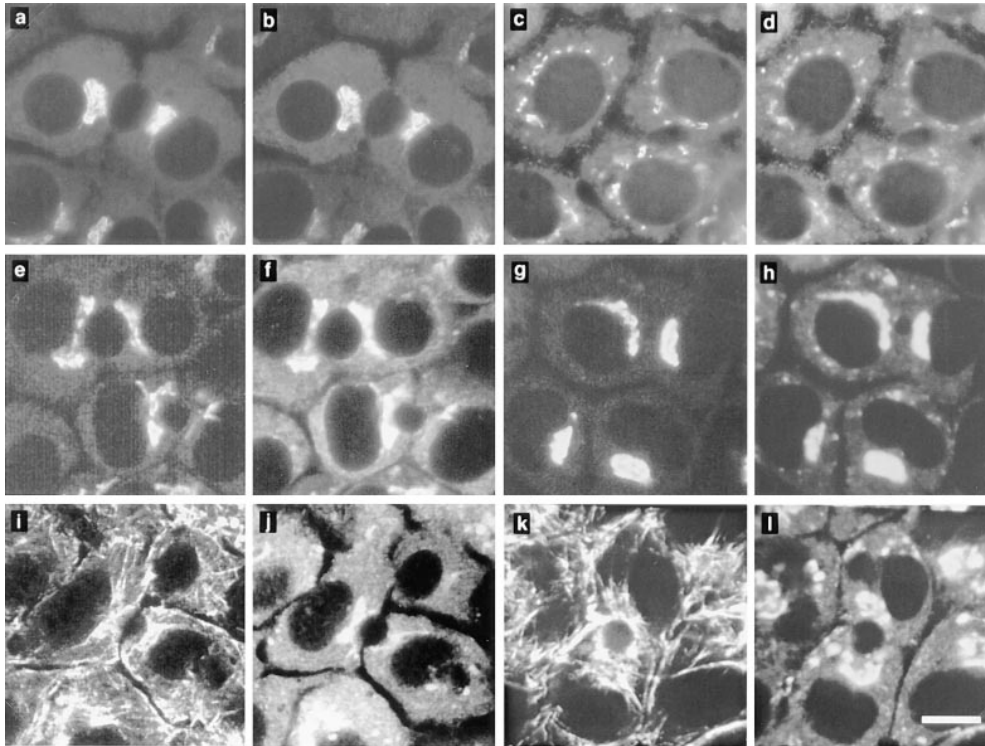
Figure 6. 201-F causes MT-dependent fragmentation of the Golgi complex. Cells were treated without ( a, b ) or with ( c, d ) 25 \mu M 201-F for 1 h, fixed, and processed for double immunofluorescence labeling using antibodies to Man II ( a, c ) and secretory albumin ( b, d ). In a second set of experiments, cells were treated with 10 \mu M taxol for 2 h in serum-free culture medium to stabilize MTs ( e, f, i, j ), or with taxol alone for 1 h and then with a mixture of taxol and 201-F for one more hour ( g, h, k, l ). After fixation, cells were subjected to double immunofluorescence labeling of Man II ( e, g ) and albumin ( f, h ), or that of \alpha -tubulin ( i, k ) and albumin ( j, l ). All samples were examined in a confocal microscope. Bar, 10 \mu m.
