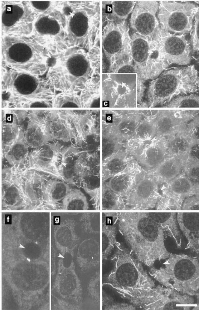
Figure 1. Effect of 201-F on the MT network of WIF-B cells. Cells grown for 8 d on glass coverslips were treated for 60 min without ( a, d, f, g ) or with 25 \mu\text{M} 201-F ( b, e, h ). 201-F treatment was extended to 4 h in c . After fixation and permeabilization for 3 min in -20^\circ\text{C} methanol, MTs were labeled using antibodies to \alpha -tubulin ( a, b, c ), acetylated tubulin ( d, e ), detyrosinated ( f ), polyglutamylated ( g ), or tyrosinated tubulin ( h ). After incubation with FITC-labeled secondary antibodies, coverslips were examined by confocal microscopy. Bile canaliculi are indicated by arrowheads. Bar, 10 \mu\text{m} .
