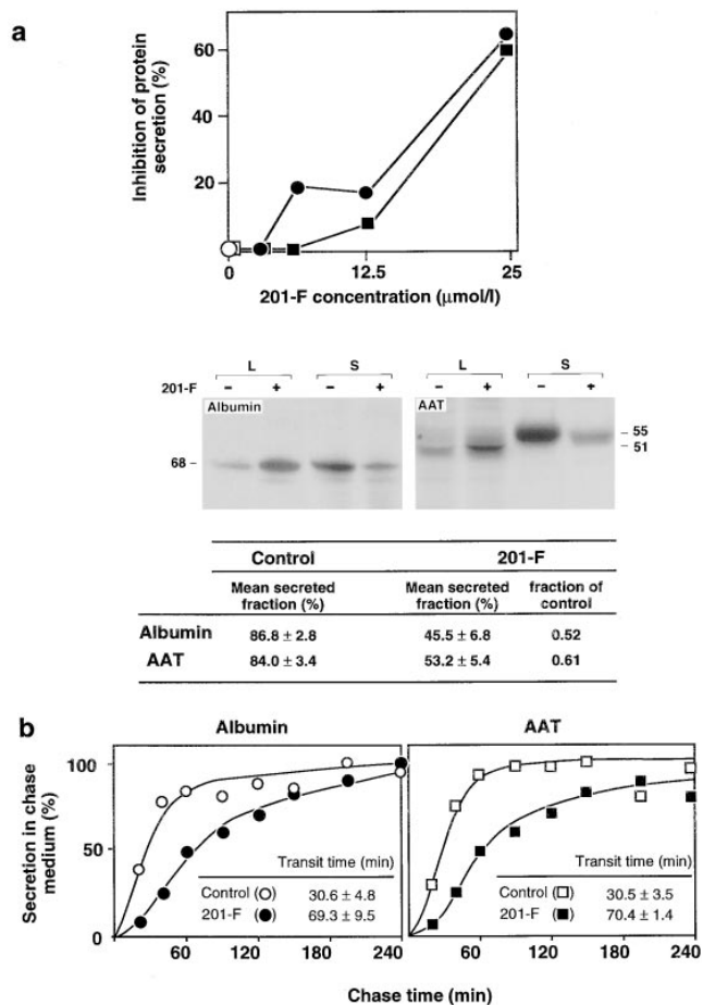
Figure 5. 201-F inhibits secretion of albumin and AAT in WIF-B cells. Cells were depleted of methionine and cysteine for 30 min, and then newly synthesized proteins were radiolabeled for 15 min with [ ^{35}\text{S} ]methionine and cysteine, and were chased for various times. When appropriate, 25 \mu\text{M} 201-F was added into the depletion, pulse, and chase media. Albumin (circles) and AAT (squares) were immunoprecipitated from cell lysates and chase supernatants, and were quantified by SDS-PAGE fluorography and densitometry. Secretion is expressed as the ratio of secreted protein to total (secreted plus intracellular) immunoprecipitated protein to normalize for the variations in the incorporation of [ ^{35}\text{S} ]methionine and cysteine. Secretion inhibition was measured relative to control values at the last chase time. (a) Effect of 201-F on albumin and AAT secretion after 1 h of chase. In the upper graph, the concentration-dependent effect of 201-F is shown. The lower part of the panel summarizes the data (mean secreted fractions \pm SEM) from four (AAT) to eight experiments (albumin), and show a sample SDS-PAGE of albumin and AAT immunoprecipitated from cell lysates (L) and chase supernatants (S). (b) Secretion kinetics of albumin and AAT in control (open symbols) and 201-F-treated cells (closed symbols). Kinetic data are fitted to a three-compartment model for secretion by a nonlinear least-square method. Transit times are the sum of the reciprocals of the two rate constants computed from experimental data; they are the mean \pm SEM of three independent determinations.
