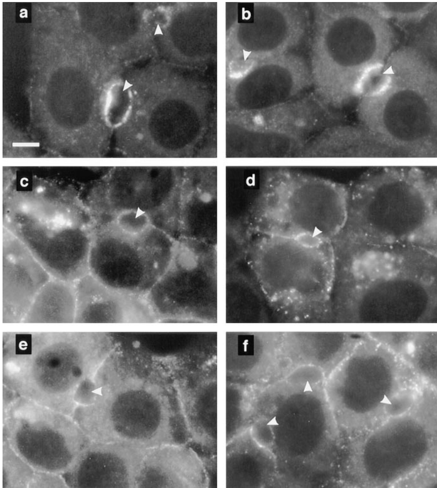
Figure 10. Dynamic MTs are involved in the transcytosis of B10 and DPP IV from the basolateral to apical surface of WIF-B cells. Control ( a, b ), 201-F-treated (2 h, 25 \mu M; c, d ) and nocodazole-treated cells (10 h, 10 \mu M; e, f ), were incubated at 37°C for 2 h with anti-DPP IV ( a, c, e ) or anti-B10 antibodies ( b, d, f ). After washing with PBS, cells were fixed, and the immune complexes were revealed using FITC-labeled secondary antibody. Cells were examined in a fluorescence microscope. Bar, 10 \mu m.
