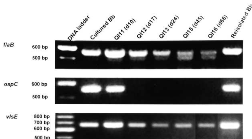
Figure 1. Selection of OspC nonexpressers as infection progresses. Five C3H mice were infected with cultured spirochetes and killed at 10 (mouse QI11), 17 (QI12), 24 (QI13), 45 (QI15), and 66 d (QI16) PI. Total RNA was purified from cultured spirochetes (cultured Bb), mouse ear tissues, or reisolated spirochetes (reisolated Bb), and analyzed by RT-PCR for expression of the flaB , ospC , and vlsE genes. PCR products were separated by ethidium bromide-incorporated-agarose gel electrophoresis.
