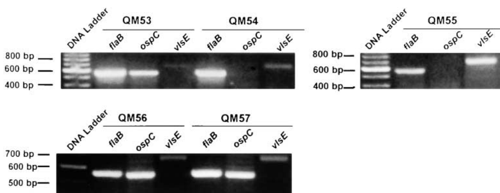
Figure 5. B. burgdorferi reexpressed ospC in passively immunized SCID mice after specific antibody was cleared. Five SCID mice were inoculated with cultured spirochetes. Mice QM54, QM55, QM56, and QM57 were passively immunized with three doses of anti-OspC monoclonal antibody at 10, 12, and 14 d PI while mouse QM53 was given IgG2a isotype control. Mice QM53 and QM54 were killed 3 d later. QM55, QM56, and QM57 received two doses of anti-mouse IgG at 5 and 7 d after
