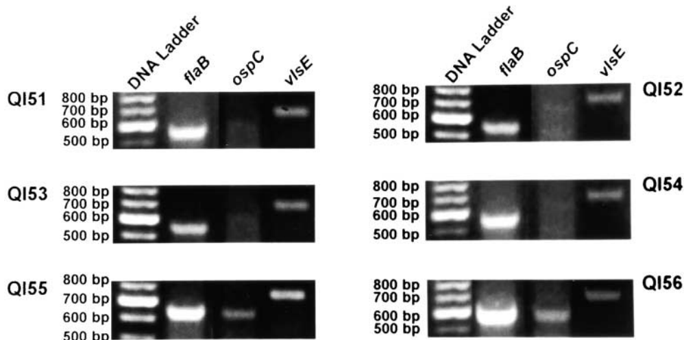
Figure 4. Passively transferred anti-OspC antibody selectively eliminated OspC-expressing spirochetes in infected SCID mice. Six SCID mice were infected with cultured spirochetes. Mice QI51 and QI52 were passively immunized with 2, 5, 10, 50, 100, and 100 \mu g anti-OspC monoclonal antibody at 10, 12, 14, 17, 19, and 21 d PI and were killed 3 d later. Mice QI53 and QI54 were passively immunized with three doses of 100 \mu g anti-OspC monoclonal antibody whereas mice QI55 and QI56 were given three doses of 100 \mu g mouse IgG2a isotype control at 17, 19, and 21 d PI and were
