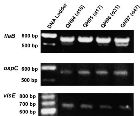
Figure 3. B. burgdorferi persistently expressed ospC in SCID mice. Four C3H-SCID mice were infected with cultured spirochetes and killed at 10 (mouse QH94), 17 (QH95), 31 (QH96), and 47 d (QH97) PI. Total RNA was purified from mouse ear tissues and analyzed by RT-PCR for expression of the genes flaB , ospC , and vlsE . PCR products were separated by ethidium bromide-incorporated agarose gel electrophoresis.
