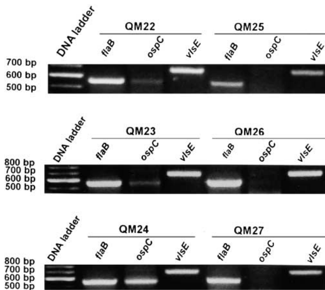
Figure 2. OspC nonexpressers reverted to expressing ospC in the absence of anti-OspC antibody but not when antibody was present. Mice QM25, QM26, and QM27 received two doses of recombinant OspC emulsified with adjuvant while QM22, QM23, and QM24 were given adjuvant alone. 10 d after the last immunization, all of the mice were inoculated with host-adapted spirochetes that had downregulated ospC . Mice QM22 and QM25 were killed at 14 d postchallenge and the rest at 18 d postchallenge. Total RNA was purified from ear tissues and analyzed by RT-PCR for expression of the genes flaB , ospC , and vlsE . PCR products were separated by ethidium bromide-incorporated agarose gel electrophoresis.
