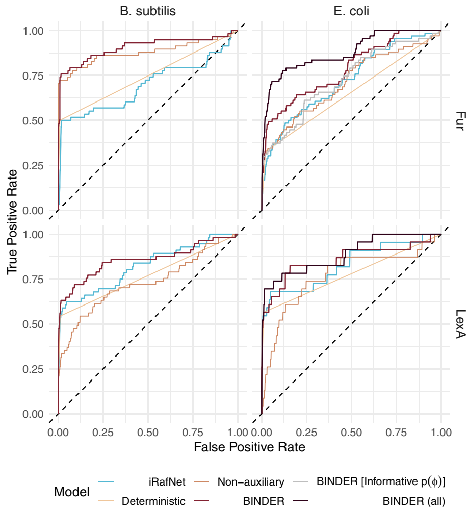
Fig. 3 ROC analysis for \theta_{r,t}^{50\%} posterior estimates for the BINDER, deterministic and non-auxiliary approaches and gene importance estimates for iRafNet for the r = fur and r = lexA regulons in E. coli and B. subtilis . BINDER (all) denotes results from analysis of BINDER applied to the complete coexpression data; BINDER relates to its application to the reduced data set
