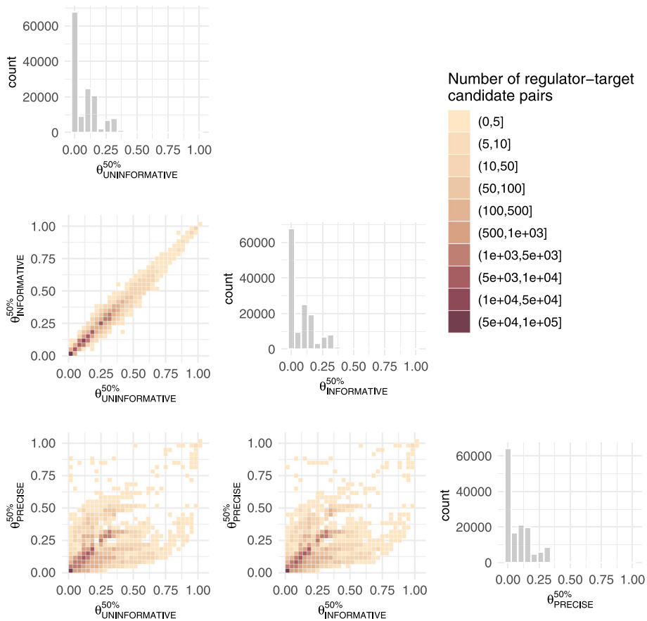
Fig. 6 Heat map illustrating the similarity between mean predicted \theta_{r,t}^{50\%} values achieved by BINDER under three distinct prior distribution parameterisations (uninformative, informative, precise) on the set of N = 167,280 regulator-target pairs
