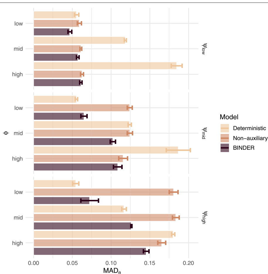
Fig. 2 Simulation results illustrating the mean absolute deviation (MAD) between the true and estimated regulation interaction probabilities achieved by the deterministic, non-auxiliary and BINDER approaches across a range of dispersion parameter settings
