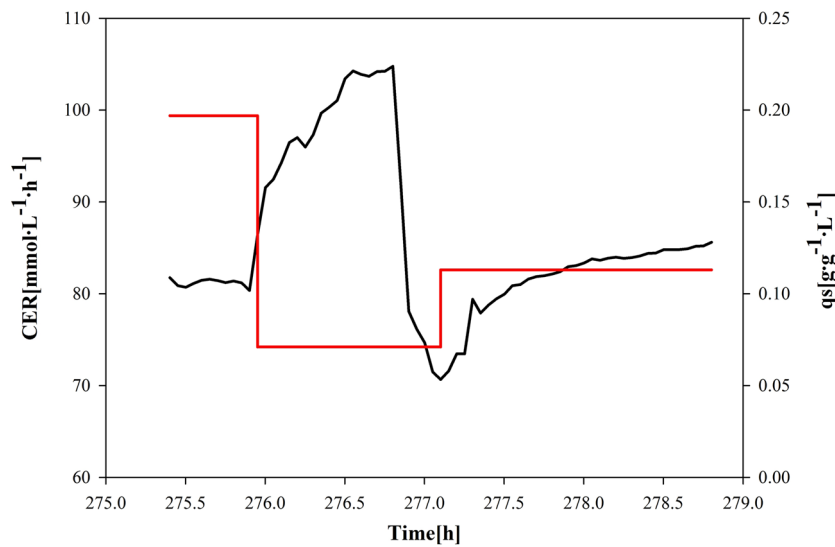
Figure 2 Glycerol pulse during sorbitol fed-batch. Carbon dioxide evolution rate (CER, continuous black line ) and specific sorbitol uptake rate ( q_{s \text{ sorbitol}} , continuous red line ). After glycerol pulse a sudden increase in the CER signal and a concomitant decrease in q_{s \text{ sorbitol}} were observed.
