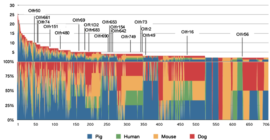
Figure 3 Comparison of OR gene similarity among humans, dogs, mice, and pigs by clustering analysis of OR genes on the basis of their amino acid sequence similarity. The names of ORs with known chemical specificity from humans and mice were indicated above the graph. The Y-axis of the upper graph shows the number of OR genes in each cluster ranging from two to 26 genes. The X-axis of both the upper and lower graphs indicates the cluster number, with 706 clusters. The Y-axis of the lower graph indicates the percentage of OR genes of each species within the cluster. The OR genes of different species are indicated by different colors. See the additional file 9 for the uncompressed original image of Figure 3.
