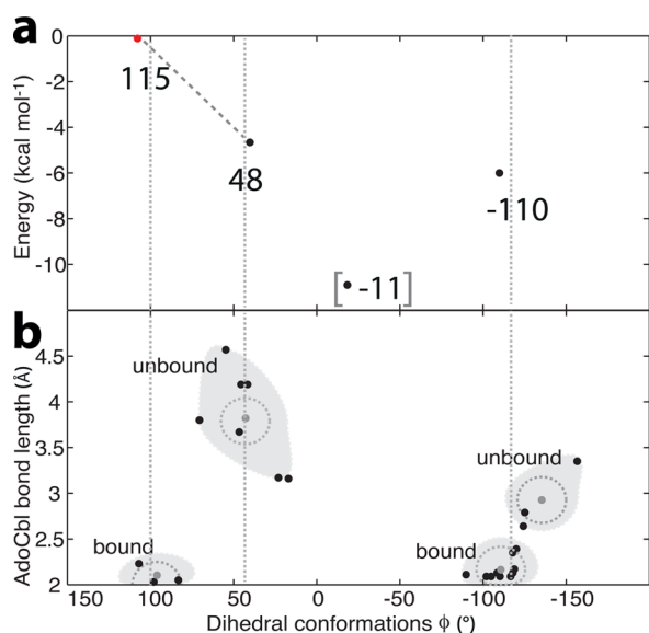
Figure 3. Different conformations of Ado \cdot in other B_{12} -dependent enzymes. In (a), the results of a relaxed scan in gas phase along glycosidic bond, the O_4-C_1-N_9-C_8 dihedral angle, of an isolated Ado \cdot moiety. The scan uncovers several free energy minimum structures: \phi of 48, -11, and -110^\circ . All energies (M06/6-31G(d)) are relative to an arbitrarily chosen origin, an orientation of Ado \cdot taken from the QM/MM simulations following AdoCbl bond cleavage (an averaged value of \phi of 115^\circ \pm 8.9 ). Performing a geometry optimization of Ado \cdot from this bound state gains nearly 5 kcal mol -1 of energy via the rotation of \phi from 115^\circ to 48^\circ (indicated by the dashed gray line connecting these two points). In (b), the \phi values taken from various B_{12} -dependent enzymes, plotted as a function of AdoCbl bond length. The gray points represent the average dihedral value for each cluster. When bound to Co(III), the value of \phi is 50-80^\circ larger than it is in the unbound state. As previously suggested, 21 the global minimum structure in the gas phase ( \phi = -11^\circ ) is stabilized by an intramolecular hydrogen bond between H-O 2 and N 3 , which is not observed in the condensed phase.
