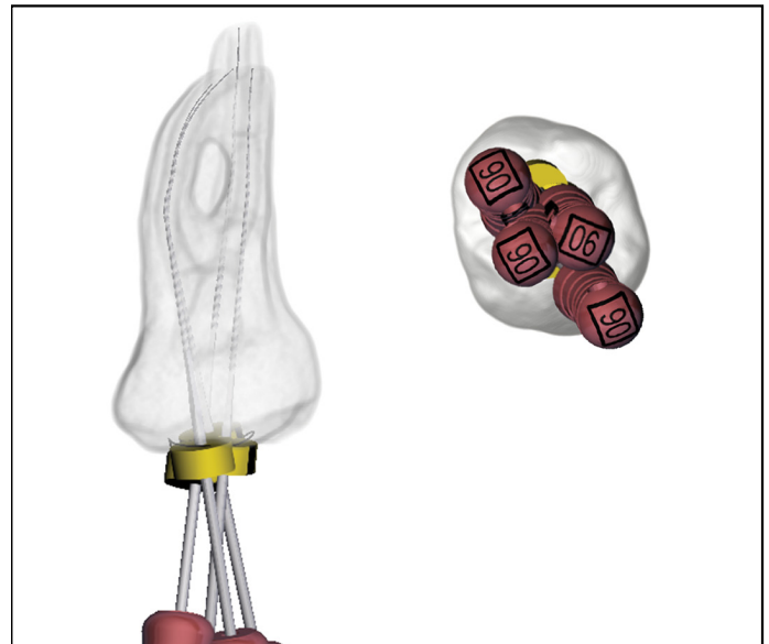
Figure 2. Overlying dentine was virtually removed by straightening the coronal part of the instrument along a tangent between the outermost pulp chamber and outer the root canal curvature
