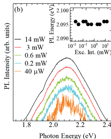
Fig. 6 (a) PL decay profiles, detected at 1.82, 2.07, and 2.33 eV, for the Cu:CdSe/ZnS at a temperature of 15 K. The PL spectrum is shown in the inset. (b) Excitation intensity dependence of PL spectra expanded in the vicinity of the peak of the Cu-PL band. The inset shows the dependence of the PL peak energy on the excitation intensity.
