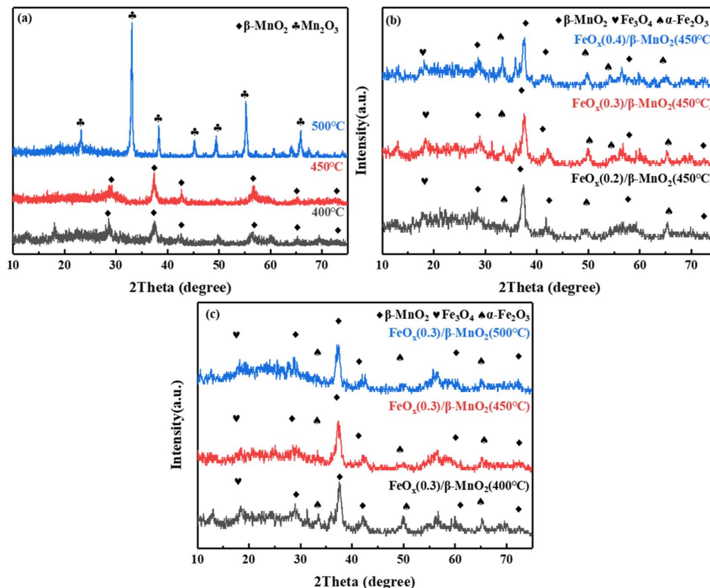
Fig. 3 XRD patterns of (a) \beta - \text{MnO}_2 at different calcination temperatures; (b) \text{FeO}_x(n)/\beta - \text{MnO}_2(450^\circ\text{C}) with different molar ratios of Fe/Mn; (c) \text{FeO}_x(0.3)/\beta - \text{MnO}_2 at different calcination temperatures.
