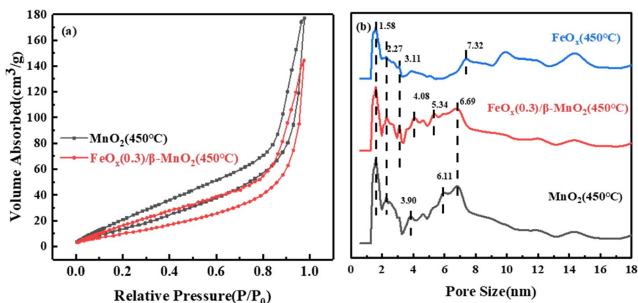
Fig. 4 (a) \text{N}_2 adsorption-desorption curve and (b) average pore size of catalysts.
