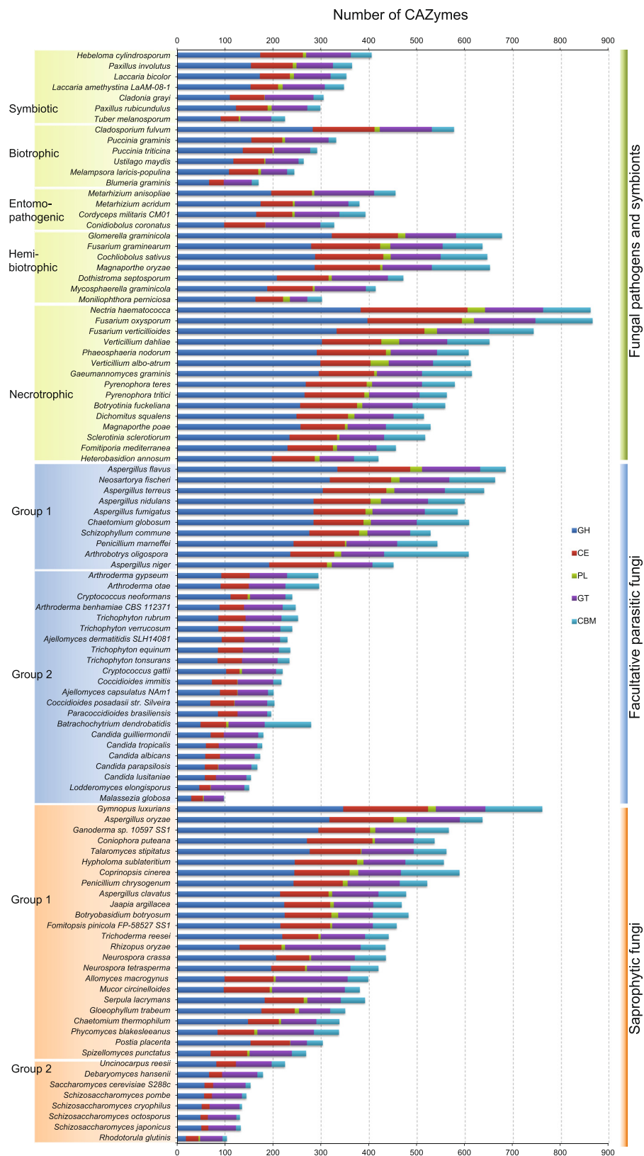
Figure 1 Comparative analysis of fungal CAZymes. The numbers of CAZyme modules or domains were represented as horizontal bars. CBM, carbohydrate binding module; CE, carbohydrate esterase; GH, glycoside hydrolases; GT, glycosyltransferase; PL, polysaccharide lyase.
