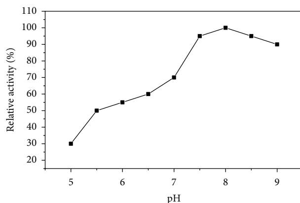
FIGURE 6: pH stability of asparaginase I from P. vulgaris at different pH after incubation for 24 h at 4°C.
