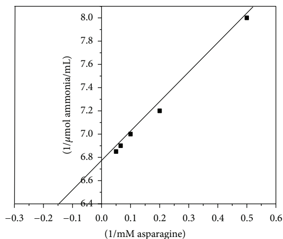
FIGURE 4: Lineweaver-Burk plot relating of asparaginase I from P. vulgaris velocities to different L-asparagine concentrations.
