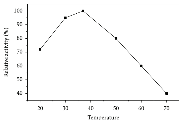
FIGURE 7: Temperature optimum of asparaginase I from P. vulgaris . The enzyme activity was measured at various temperatures using the standard assay method as previously described.
