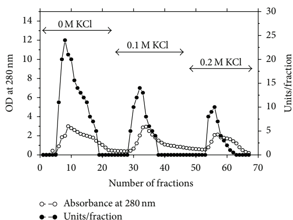
FIGURE 1: A typical elution profile for the chromatography of asparaginase from P. vulgaris on DEAE-Sepharose column ( 15 \times 1.6 cm i.d.) previously equilibrated with 20 mM Tris-HCl buffer, pH 8.0 at a flow rate of 60 mL/h and 3 mL fractions.
