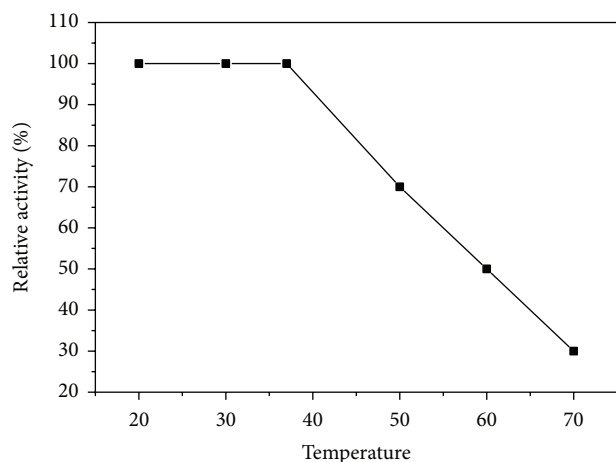
FIGURE 8: Thermal stability of asparaginase I from P. vulgaris . The reaction mixture was preincubated at various temperatures for 60 min prior to substrate addition, followed by cooling in an ice bath. The enzyme activity was measured using the standard assay method as previously described. Activity at zero time was taken as 100% activity.
