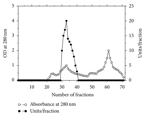
FIGURE 2: Gel filtration of asparaginase I from DEAE-Sepharose fraction on Sephacryl S-200 column ( 90 \times 1.6 cm i.d.). The column was equilibrated with 20 mM Tris-HCl buffer, pH 8.0 at a flow rate of 30 mL/h and 3 mL fractions.
