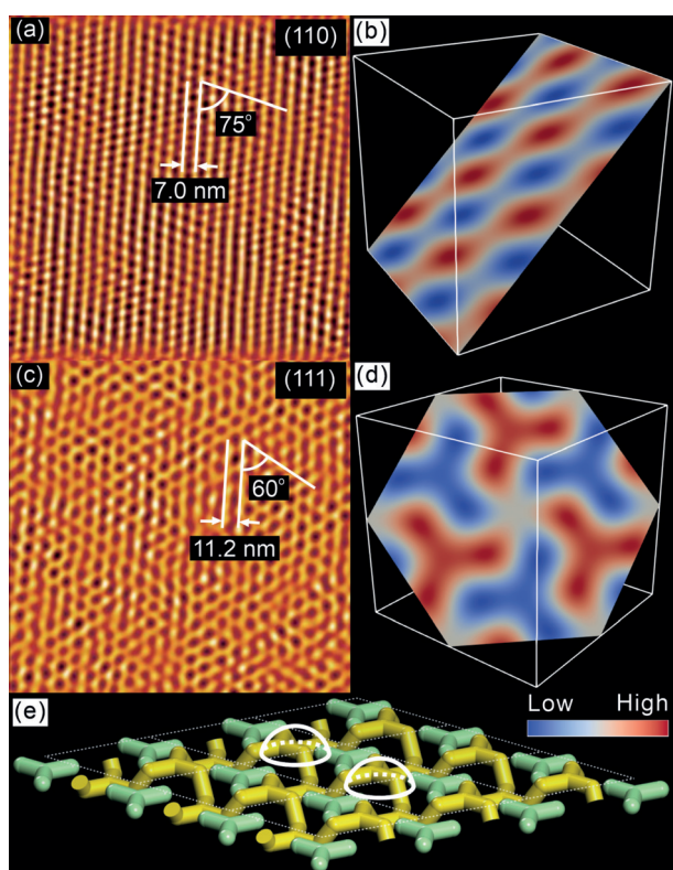
Figure 3. AFM phase images of the I4_32 phase of compound 3 recorded at 40°C after cooling in situ from 110°C (Iso) to 90°C at 0.5 Kmin -1 and then at 3 Kmin -1 to 40°C. a) a (110) plane, c) a (111) plane (Fourier filtered). b and d show (110) and (111) cuts, respectively, through an electron density map (the 2 \times 2 \times 2 = 8 unit cell box). See also frontal view of b) with marked dimensions in Figure S14. e) Model of the surface layer of unit cells showing network segments as rods. The white domes are the suggested blobs of aggregated R_f chains seen as dark dots in (c).
