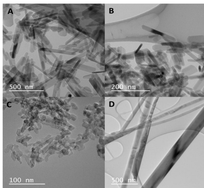
Figure 1. Hydroxyapatite nanoparticle (HANP) transmission electron microscopy (TEM) micrographs of the long rods (A), sheets (B), dots (C), and fibers (D).
