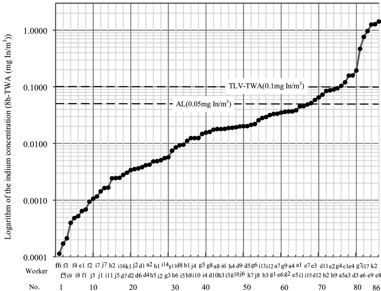
Fig. 1. Individual 8h-TWA indium total dust exposure concentrations of the 86 workers. The individuals are identified by a number and a letter, which indicates the plant where they were employed. The two dashed lines indicate the TLV-TWA (0.1 mg/m 3 ) and the AL (0.05 mg/m 3 ).
