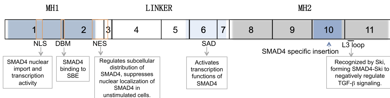
Figure 1 The schematic diagram to show the structure of SMAD4. SMAD4 is composed of three different domains, MH1, linker region and MH2 domain. Nuclear localization signal (NLS), DNA binding motif (DBM) and nuclear export signal (NES) are in MH1 domain. And linker region has a Smad-activation domain (SAD). In MH2 domain, there is a region that is called SMAD4 specific insertion and MH2 mutation often occur in this region. L3 loop of MH2 domain is important for forming complex with R-Smads.
