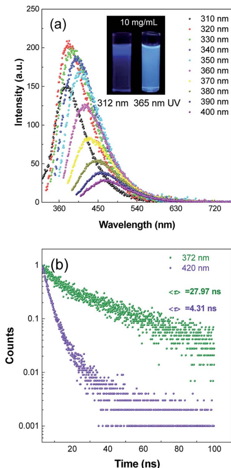
Fig. 1 (a) Fluorescence spectra of PASAS aqueous solution ( 10 \text{ mg mL}^{-1} ) with different excitation wavelengths. (b) The effect of excitation wavelength on fluorescence lifetimes of PASAS aqueous solution ( 10 \text{ mg mL}^{-1} ).
