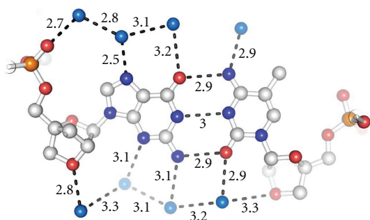
FIGURE 3: Hydration pattern within the LNA duplex (PDB ID: 2X2Y): a region of the LNA helix showing the base pair (G4-m 5 C69) l . The hydration pattern resembles that known for RNA, as the bridged 2'-oxygen atom in LNA acts as a hydrogen bond acceptor similar to the 2'-oxygen in the hydroxyl group of RNA.
