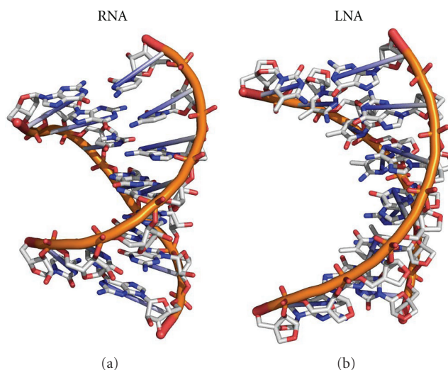
FIGURE 2: Crystal structure of the RNA duplex r[GGUGAGG]·r[CCUCACC] (PDB ID: 3GVN) as compared to the corresponding LNA helix (PDB ID: 2X2Y).
