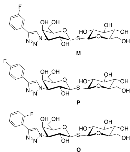
Figure 1. Chemical structures of the three fluorinated phenyltriazolyl-galactosylthiogluco-sides galectin-3C ligands M, P, and O.
