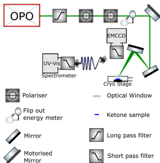
Fig. 1 The optical pathway for the excitation and emission detection for the samples in the cryogenic stage
