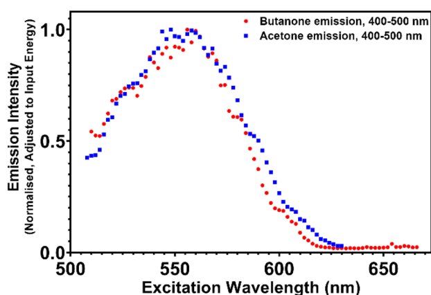
Fig. 2 Excitation spectra of acetone and butanone, frozen at 163 K. Emission was collected from 400–500 nm
