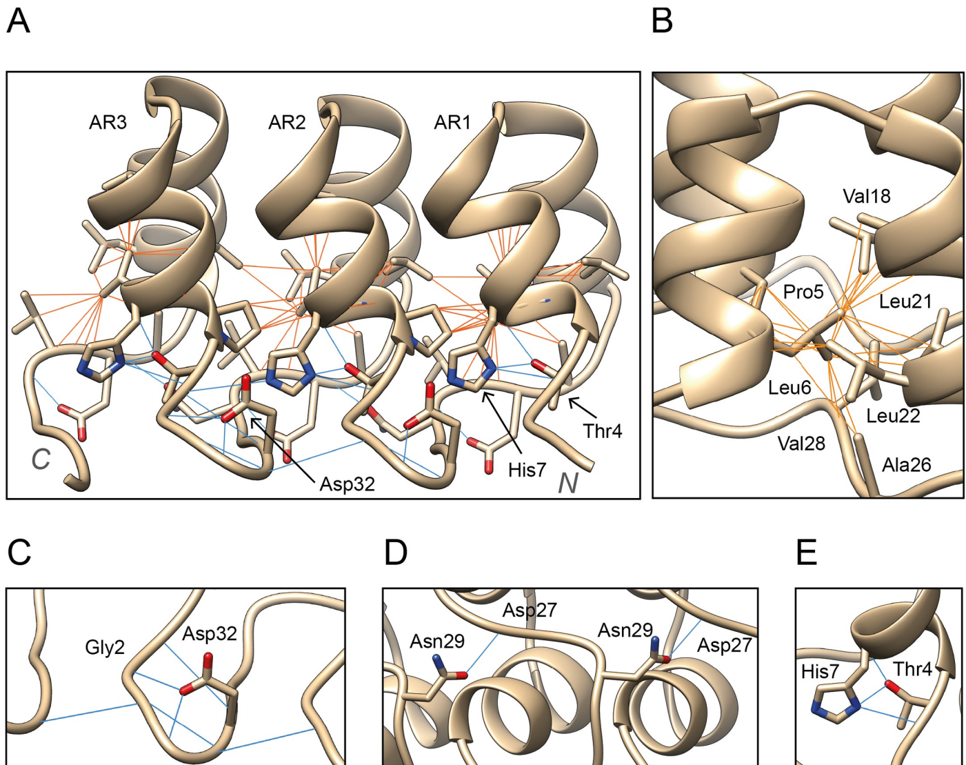
Fig 2. (A) Trio of ARs from a designed ankyrin repeat protein [14] (PDB: 5MA3). These three ARs display the main interactions responsible for the correct packing of the ARD. Hydrogen bond interactions are depicted by blue lines whereas hydrophobic ones are depicted in orange; (B) Hydrophobic network formed by Leu6 in the hydrophobic core of the domain; (C) Hydrogen bonding network at the \beta -turn between positions Asp32-Gly2; (D) Inter-repeat hydrogen bonds between conserved Asn29 and Asp27; (E) Thr4 forms three hydrogen bonds with His7. Structure visualization with UCSF Chimera [7].
