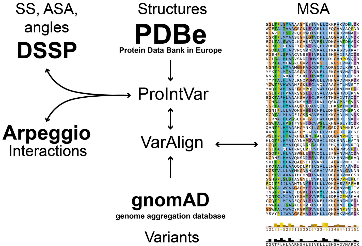
Fig 5. Diagram showing the main components of the pipeline. VarAlign retrieves variants found in human sequences in the MSA from gnomAD. ProIntVar retrieves structures from the PDBe and runs DSSP and Arpeggio to get secondary structure, accessible surface area and inter-atomic contacts information. Everything is mapped back to the residues and MSA columns [40].
