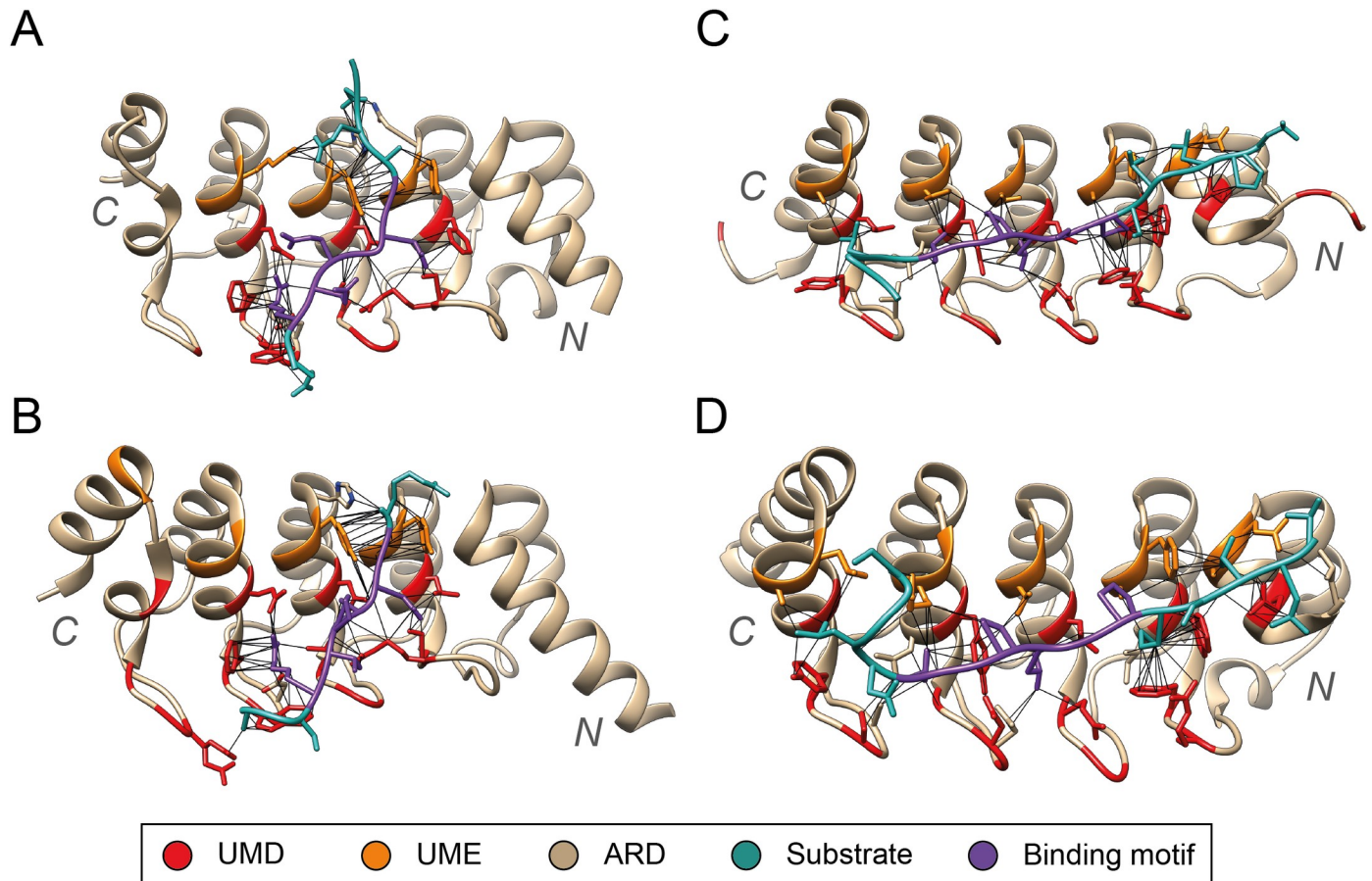
Fig 12. ARDs in complex with substrates. (A) RFXANK and RFX5 (PDB ID: 3V30) [56]; (B) ANRA2 and HDAC4 (3V31); (C) TNKS2 and ARPIN (4Z68) [59]; (D) TNKS1 and USP25 (5GP7) [60]. UMD positions (red) and UMEs 11, 12 (orange) are conserved across proteins that bind similar substrates (dark cyan). For example, these positions are conserved across TNKS2 and TNKS1, which are known to bind substrates with the motif RXXPDG (purple). Similarly, RFXANK and ANRA2, bind substrates with the motif PXLPX[I/L] (purple). Figure obtained with UCSF Chimera [7].
