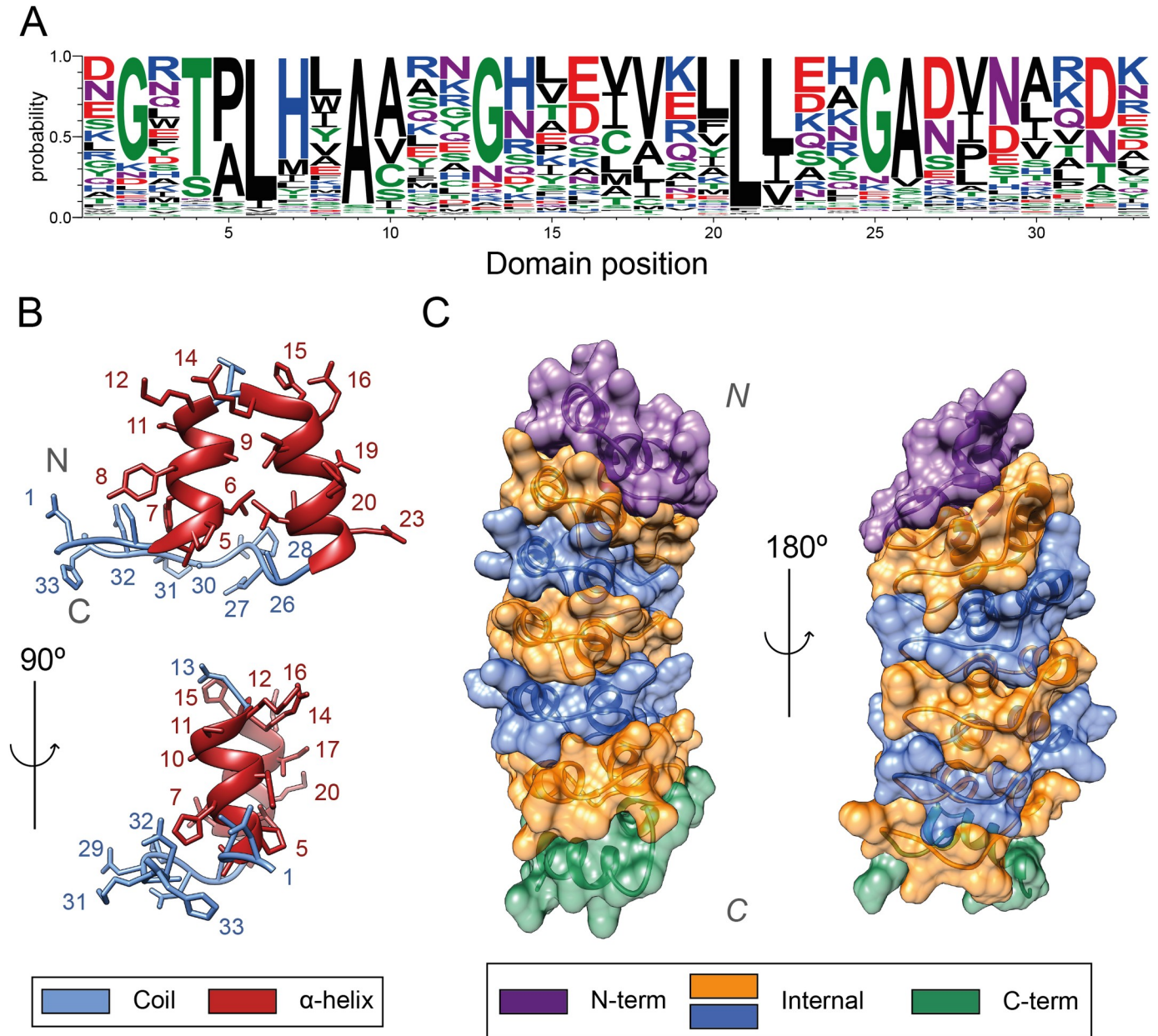
Fig 1. (A) Sequence logo of the ANK obtained with WebLogo [5] derived from the MSA generated in this work. The Y axis indicates the probability of observing an amino acid at any position within the motif; (B) Tertiary structure of an ankyrin repeat, coloured by secondary structure class: helices in red and coil in blue; (C) Representation of the complementary surfaces of individual ARs that form the human gankyrin ARD surface. N- and C-capping AR surfaces are coloured in purple and green respectively, whereas internal ones are coloured in blue and orange. (PDB ID: 1UOH) [6]. Structure visualization with UCSF Chimera [7].
