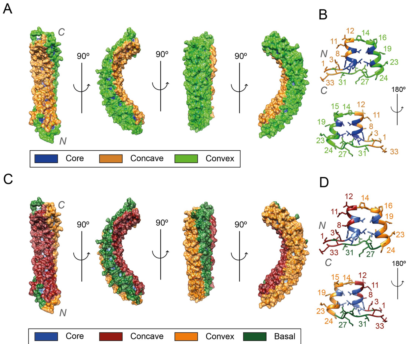
Fig 8. Comparison of the original definition of the ARD surfaces (A, B) with the new definitions derived from the results of this study (C, D). All panels refer to the D34 region of ANK1 ARD, PDB accession: 1N11 [53]. This structure shows 12 out of the 23 ARs found on this ARD; (A) Surface of an ARD. Residues conforming the concave surface are coloured in orange, residues on the convex surface in green and buried residues in blue; (B) Structure of an individual repeat. The first \alpha -helix and the \beta -turn region form the concave surface, whereas the second helix and the loop form the convex one; (C) Residues forming the concave surface are coloured in dark red, residues on the convex surface in orange, the basal surface is coloured on dark green and buried residues in blue; (D) Structure of an individual repeat with new surface classification. Figure obtained with UCSF Chimera [7].
