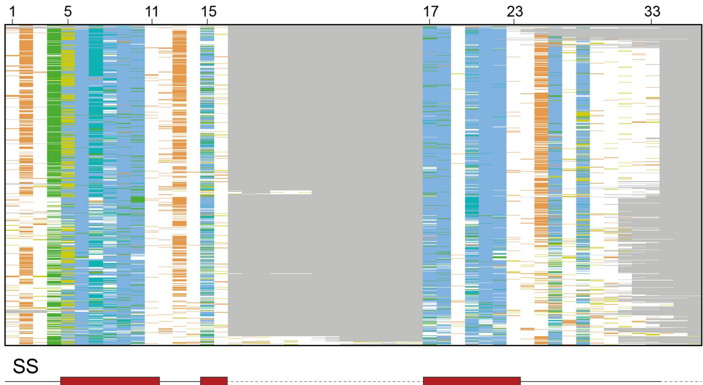
Fig 4. Overview of the resulting MSA, including the 7,404 ankyrin repeat sequences. Only columns with occupancy > 0.5% are shown. Sequences are sorted by a tree generated in Jalview using the average distance method and the BLOSUM62 matrix. Columns between 16–17 and after 33 represent insertions in some ankyrin repeats. Red boxes below the overview indicate the location of the secondary structure elements (SS), \alpha -helices in this case, within the alignment. Grey dashed lines represent gaps and are mostly found at low-occupancy columns. Columns are coloured according to the ClustalX colour scheme [34]. Hydrophobic residues are coloured in blue, glycines in orange, prolines in yellow, polar residues in green and unconserved columns are coloured in white. Obtained with Jalview [35].
