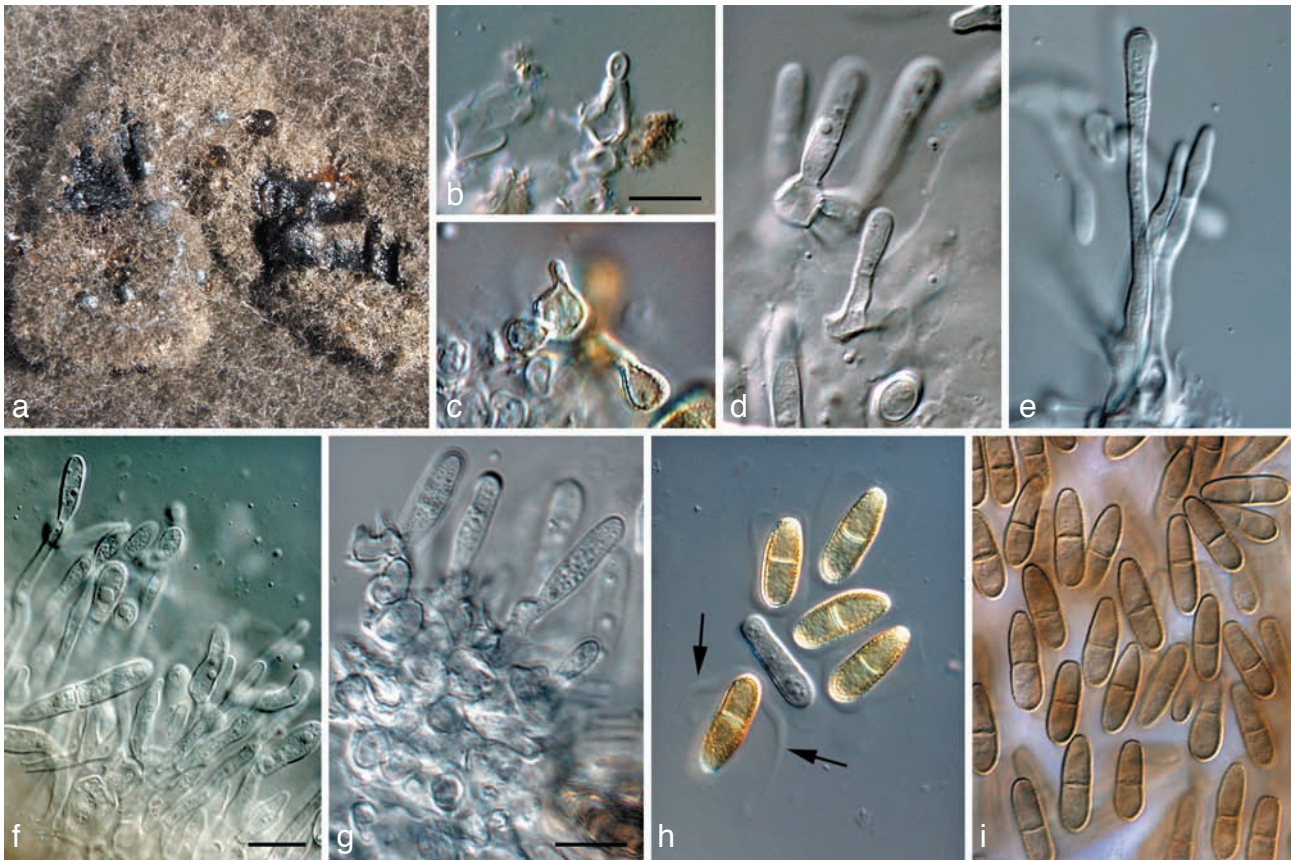
Fig. 21 Gordonomyces mucovaginat (PREM 59592). a. Colony sporulating on PDA; b–d, g. conidiogenous cells giving rise to conidia; e, f. paraphyses; h. conidia with mucoid appendages (arrows); i. mature conidia. — Scale bars = 10 \mu m.
