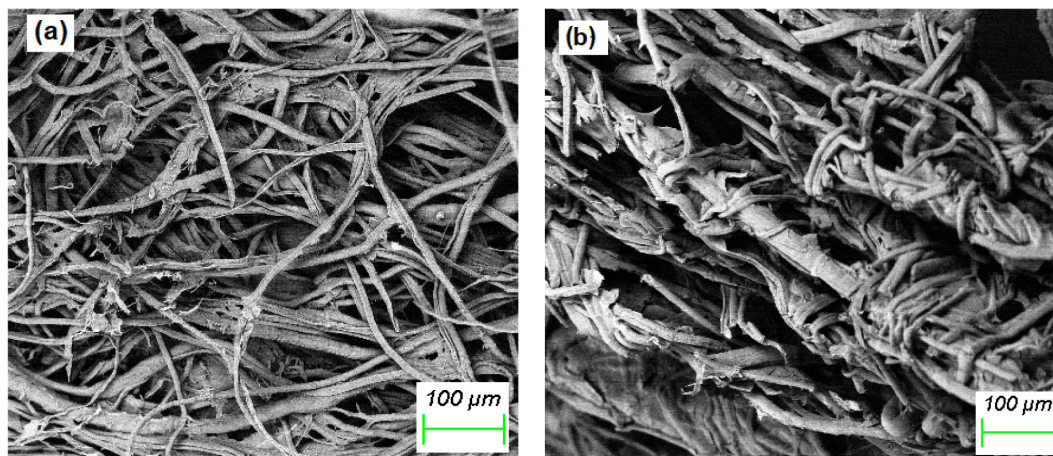
Figure 1. Scanning electron micrographs of (a) CH-cellulose, and (b) GT-cellulose.
