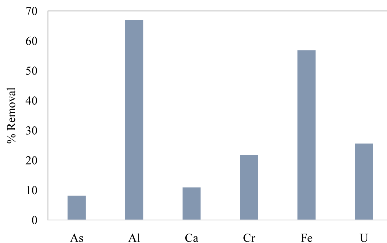
Figure 5. Removal of Cr(VI) and other ions present in mine drainage contaminated water by GT-cellulose. Conditions: pH = 2.7, adsorbent mass = 0.1 g, Volume = 20 mL, contact time = 240 minutes.
