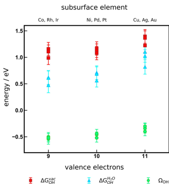
Figure 2. Adsorption energies of 1/3 ML *OH in vacuum (red, \Delta G_{OH}^{vac} ), within the water bilayer (blue, \Delta G_{OH}^{H_2O} ), and in the solvation energy (green, \Omega_{OH} ), as a function of the number of valence electrons of the subsurface metal atom in the Pt NSAs. The error bars cover the energy range spanned by the different functionals analyzed. The correlation between the number of valence electrons and the d-band centers of the Pt skins is provided in Figure S1.
