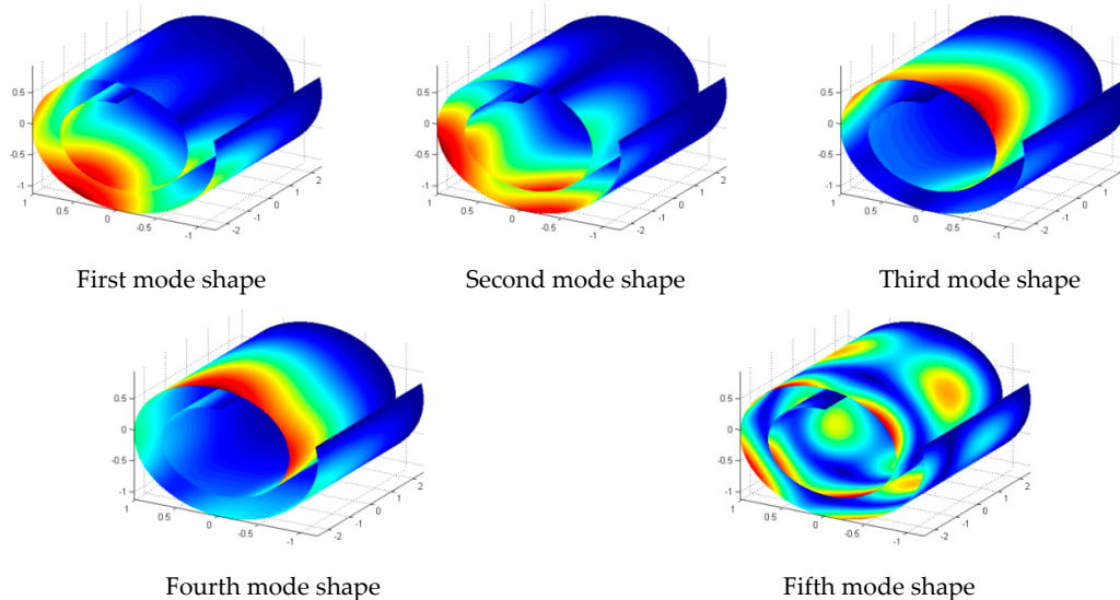
Figure 4. First five mode shapes of the CNS with FCSS boundary condition.
