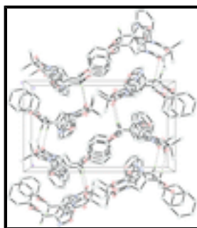
Fig. 2. Part of the crystal structure of the title compound viewed along the a axis. H atoms not involved in intermolecular interactions (dashed lines) have been omitted for clarity.
