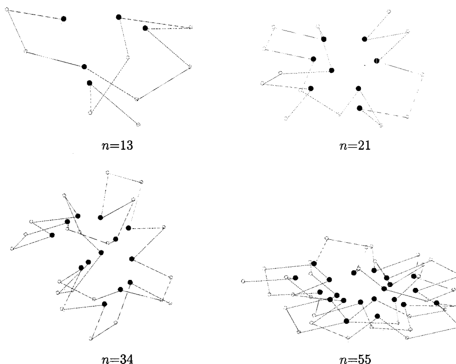
Fig. 1 Stereographic views of putative ground states of the four Fibonacci sequences listed in Table 1. Full dots and empty circles indicate hydrophobic and hydrophilic monomers, respectively.
