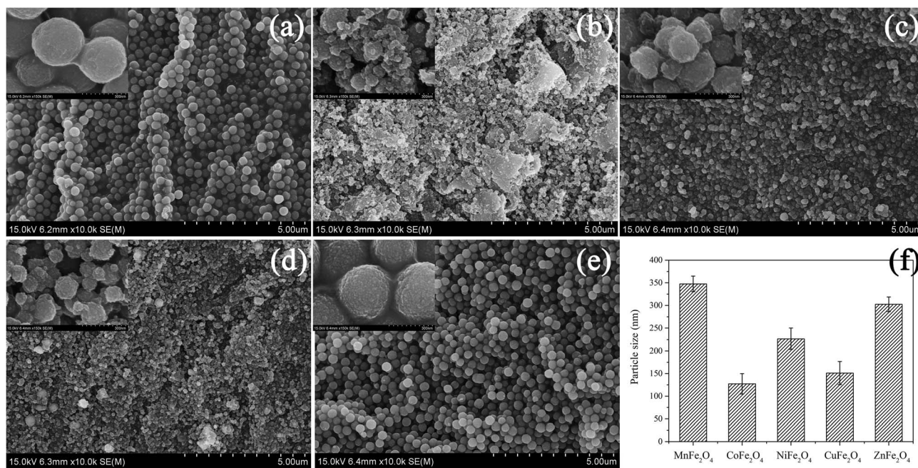
Fig. 2 SEM images of MFe_2O_4 : (a) MnFe_2O_4 , (b) CoFe_2O_4 , (c) NiFe_2O_4 , (d) CuFe_2O_4 and (e) ZnFe_2O_4 (f) size distributions of MFe_2O_4 nanoparticles.
