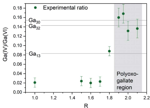
Fig. 7 Experimental ratios of the tetrahedrally to octahedrally coordinated Ga 3+ determined by 71 Ga NMR. The horizontal lines indicate the ratios in the Ga 13 , Ga 30 and Ga 32 structures at 0.083, 0.154 and 0.143 respectively. The grey area marks the R -region with the highest PDF signal from the polyoxogallate structure.
