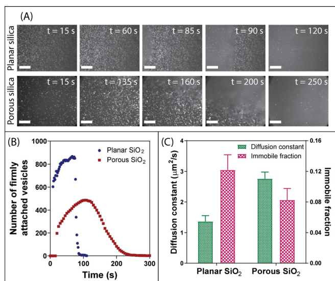
Figure 1. A) TIRF micrographs contrasting the rate and behavior of SLB formation on a planar silica substrate versus MSTF (Scale bars = 20 \mu\text{m} ). B) Time-induced changes in the number of vesicles adsorbed per 100 \times 100 \mu\text{m}^2 to a planar silica substrate (blue dots) versus MSTF (red squares) during the formation of SLBs. C) Variations in lipid membrane diffusion constant (green bars, left axis) and relative immobile fractions (pink checkered bars, right axis) for SLBs on planar and MSTF substrates. Data represents mean \pm S.D. ( n = 3 ).
