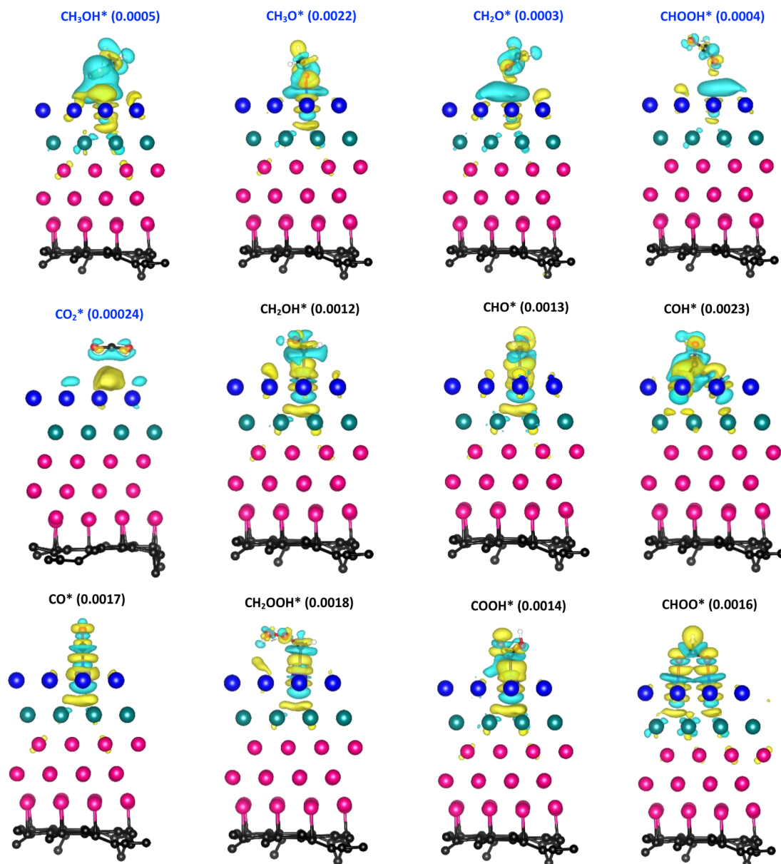
Fig. 5 The charge density difference of the systems of the adsorbed intermediate on the PtRuCo 3 /C-MWCNT substrate. The isosurface values are inside parentheses, with the unit being e^- \text{Å}^{-3} .
