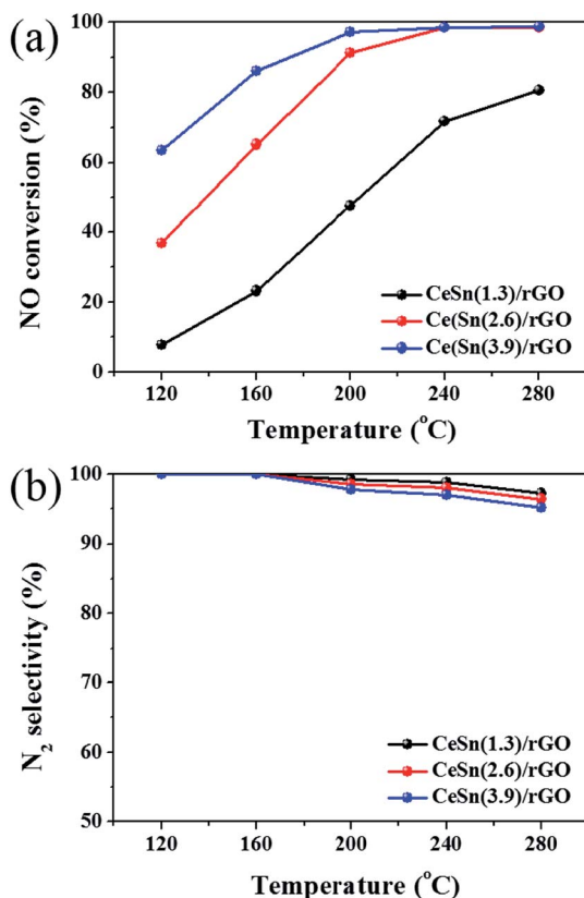
Fig. 2 NO conversions (a) and \text{N}_2 selectivity (b) over \text{CeO}_2\text{-SnO}_x/\text{rGO} catalysts with different mass ratios of (\text{Ce} + \text{Sn})/\text{GO} .
