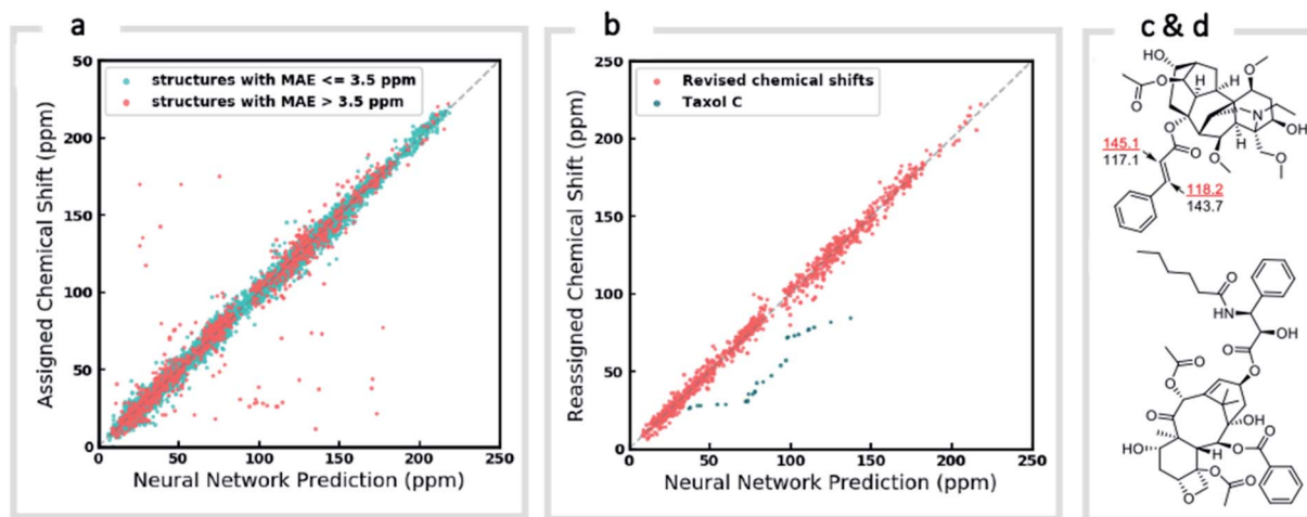
Fig. 6 Screening and revising misassignment in NMRShiftDB. (a) Correlation between predicted and experimental 13 C chemical shifts for large molecules (MW > 500). Outliers (red), here defined as structures with an MAE > 3.5 ppm, are investigated for possible misassignments (b) experimental chemical shifts for reordered assignments of outlying structures. The remaining outliers (green) helped us to identify an incorrect structure for Taxol C in the database. (c) Incorrectly assigned enoate carbons were corrected for leueantine A. (d) The correct structure of Taxol C.
