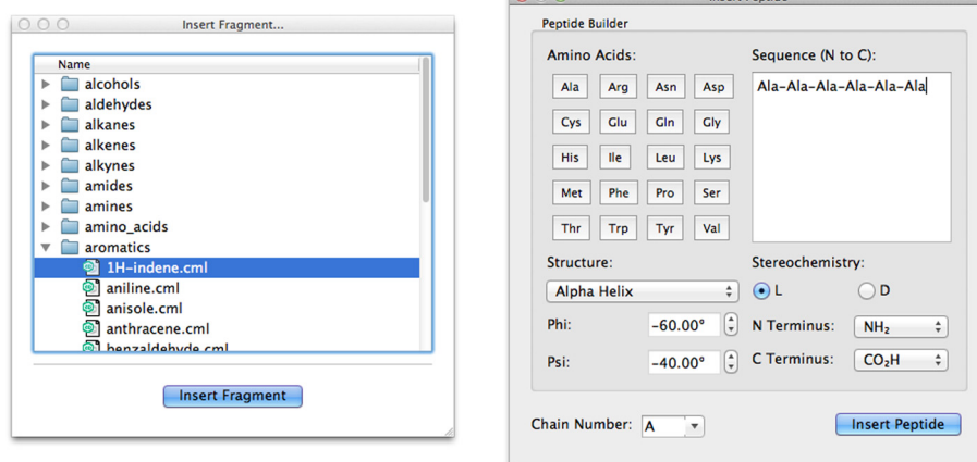
Figure 5 Dialogs for inserting pre-built fragments. The left shows molecules, and the right amino-acid sequences.
