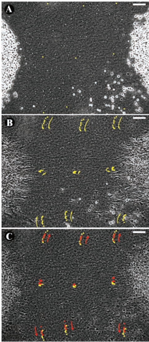
Figure 4. Collagen rearrangements during strap patterning.
