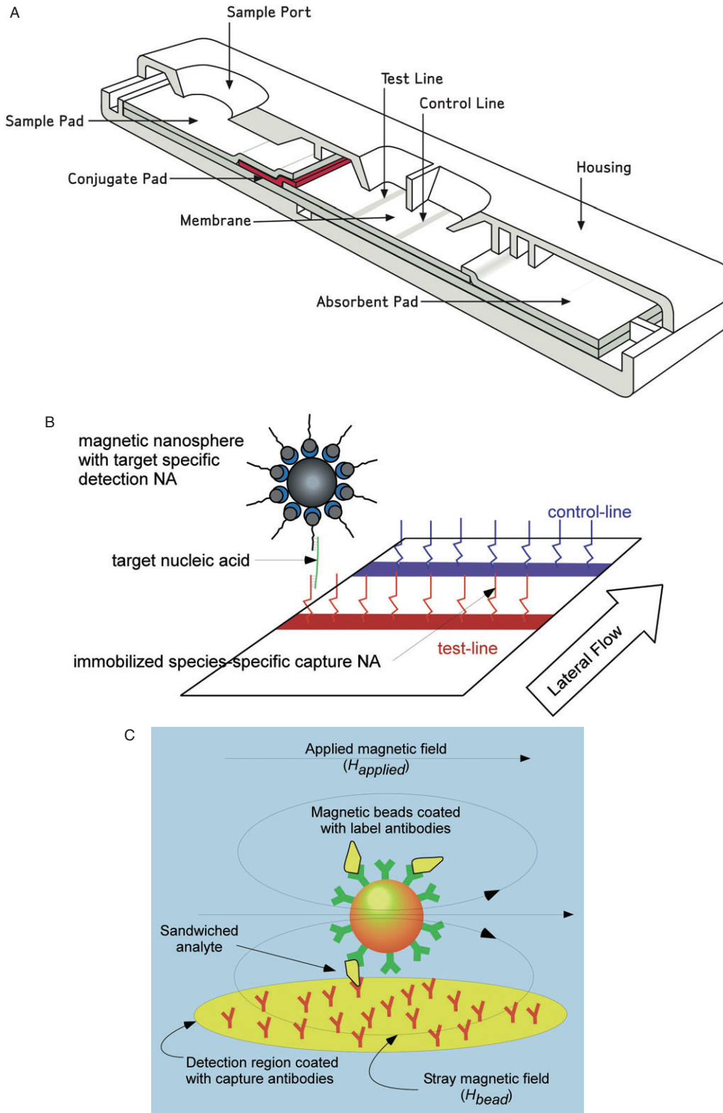
Fig. 2. A. Schematic outline of a standard lateral-flow assay device (Carney et al. , 2006). B. Lateral-flow assay of sRNA captured by PNAs using superparamagnetic magnet nanoparticles. C. Magneto-resistive detection of captured magnet nanoparticles (Tondra, 2007).
