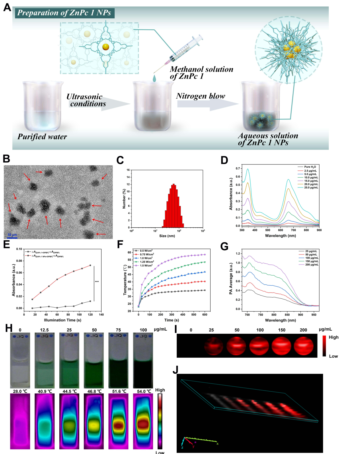
Figure 2 (A) Preparation of ZnPc I NPs. (B) TEM images of ZnPc I NPs (The red arrow in (B) indicates that ZnPc I NPs are a spherical nanoparticle). (C) Size distribution of ZnPc I NPs. (D) UV-Vis absorption spectra of ZnPc I NPs. (E) The corresponding relative absorbance variations of different groups ( \Delta A_{(ZnPc\ I\ NPs+DPBF)} - \Delta A_{(DPBF)} and \Delta A_{(ZnPc\ I\ NPs)} - \Delta A_{(DPBF)} ) at different irradiation times under the 690 nm laser irradiation (0.2 W/cm 2 ). (The three asterisk indicators in \epsilon indicate an extremely significant statistical difference in the relative absorbance variations of different groups ( \Delta A_{(ZnPc\ I\ NPs+DPBF)} - \Delta A_{(DPBF)} ) and ( \Delta A_{(ZnPc\ I\ NPs)} - \Delta A_{(DPBF)} ) under 690 nm laser irradiation (0.2 W/cm 2 ). ***) p < 0.001 as compared with the control. (F) Temperature elevation of ZnPc I NPs in dependence of power density (808 nm). (G) PA spectrum of ZnPc I NPs. (H) Optical graphs and IR thermal images of ZnPc I NPs at different concentrations (808 nm, 1.0 W/cm 2 ). In vitro (I) 2D- or (J) 3D-PA images (render) of ZnPc I NPs upon excitation wavelength at 710 nm at corresponding concentrations.
