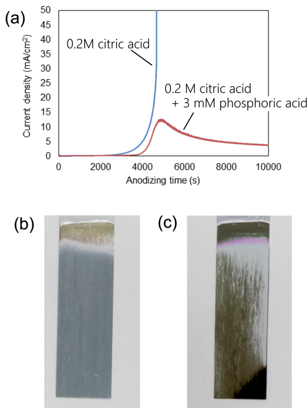
Fig. 1 (a) Current–time curves obtained during the anodization of an Al sheet in 0.2 M citric acid electrolytes with and without 3 mM phosphoric acid at 10 °C. Photographs of samples obtained in 0.2 M citric acid electrolytes with (b) and without (c) 3 mM phosphoric acid.
