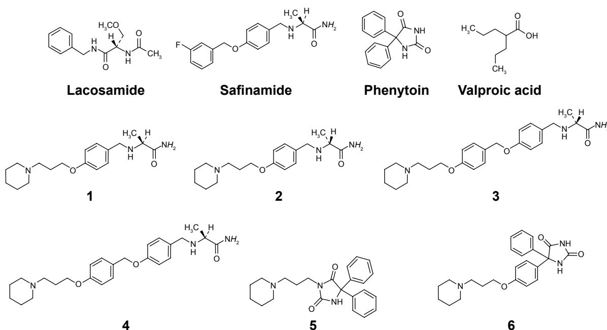
Figure 1 Structures of considered AEDs and of newly designed final compounds 1–6. Abbreviation: AEDs, antiepileptic drugs.
