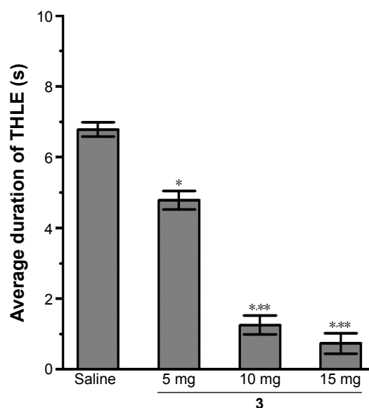
Figure 3 Dose-dependent protective effect of H 3 R ligand 3 against MES-induced convulsions.
