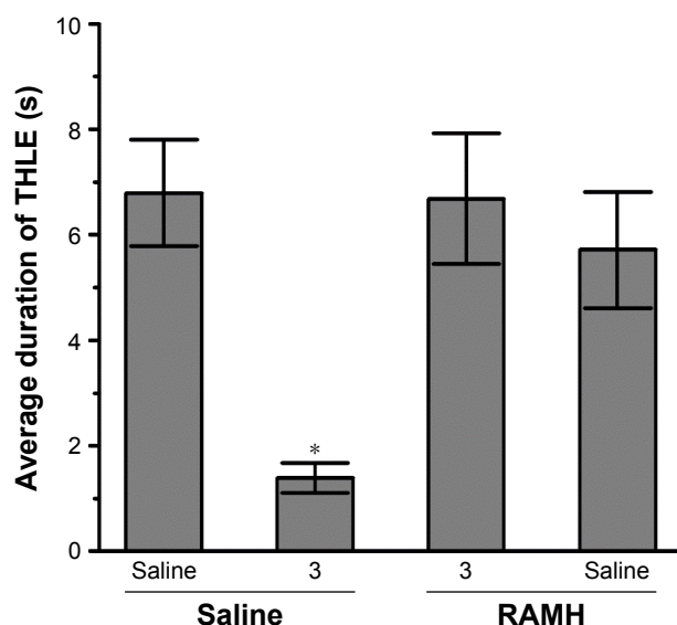
Figure 4 Effect of RAMH (10 mg/kg, IP) pretreatment on the protection by H 3 R ligand 3 (10 mg/kg, IP) on MES-induced convulsions.
