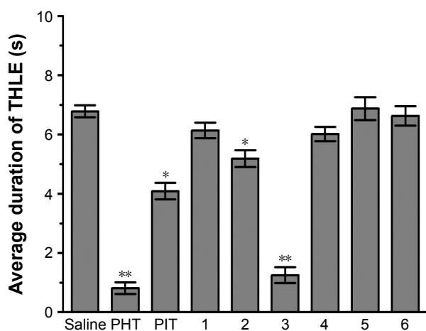
Figure 2 Protective effect of acute systemic injection of H 3 R ligands 1–6 on MES-induced convulsions in rats.
