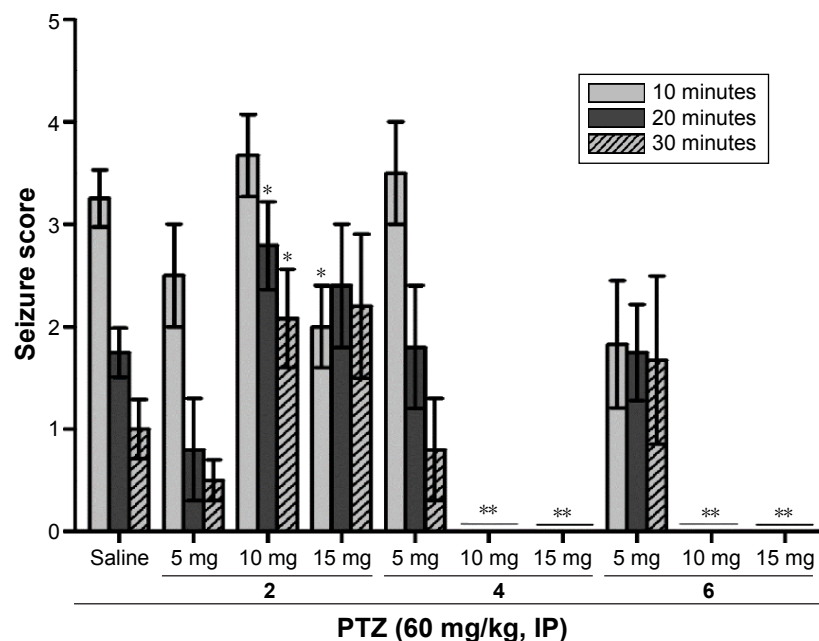
Figure 6 Dose-dependent protective effect of H_3R ligands 2 , 4 , and 5 against PTZ-induced convulsions.
