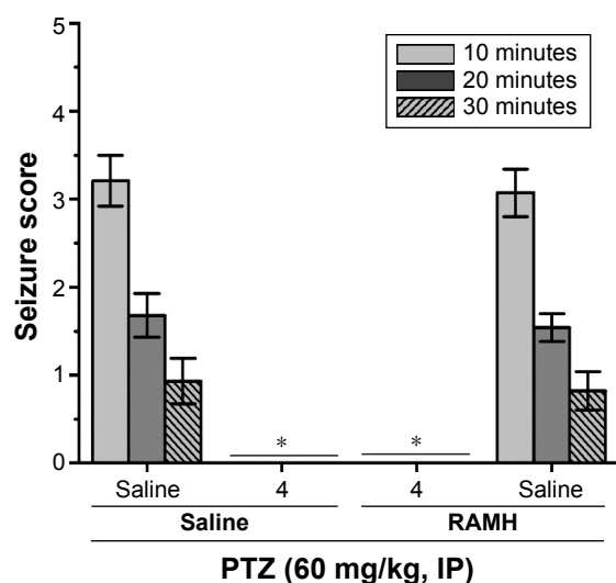
Figure 7 Effect of RAMH (10 mg/kg, IP) pretreatment on the protection by H_3R ligand 4 (10 mg/kg, IP) on PTZ-induced convulsions in rats.
