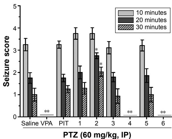
Figure 5 Protective effect of H 3 R ligands 1–6 pretreatment on PTZ-induced convulsions in rats.
