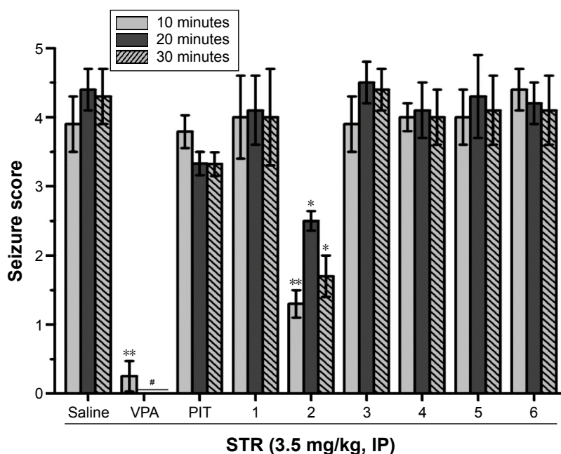
Figure 8 Protective effect of H 3 R ligands 1–6 pretreatment on STR-induced convulsions in rats.
